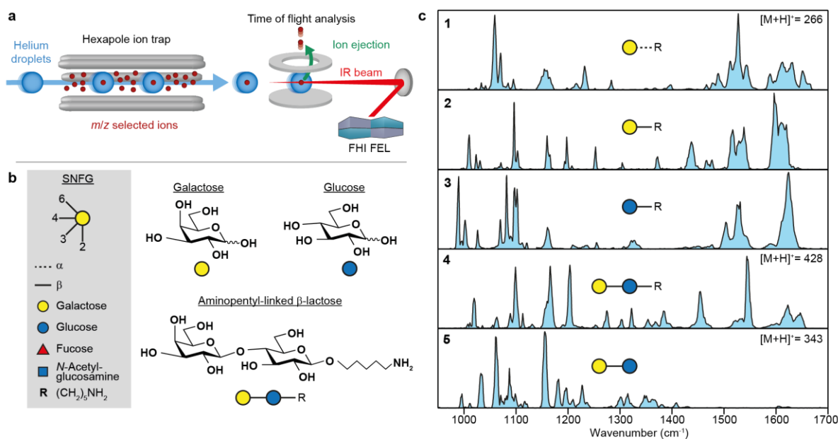
Figure 1. a, Schematic diagram of the experimental setup. Ions in the gas phase are mass-to-charge selected and accumulated inside an ion trap. Traversing helium droplets can pick up trapped ions, which immediately cools them to 0.37 K. Subsequently, the doped droplets are irradiated with IR radiation of a defined wavelength using the free-electron laser. b, representative structures of carbohydrates investigated in this work and their corresponding symbol nomenclature for glycans (SNFG) that is used throughout this article. [11] c, IR spectra of aminoalkyl-linked mono- and disaccharides \alpha -galactose 1 , \beta -galactose 2 , \beta -glucose 3 , \beta -lactose 4 and free lactose 5 , investigated as [\text{M}+\text{H}]^+ -ions.
