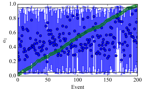
FIG. 13. For all events, median value of the primary BH spin with 90% CI. The empty green diamonds indicate the true spins. The two horizontal black lines are at 0.05 and 0.95.
