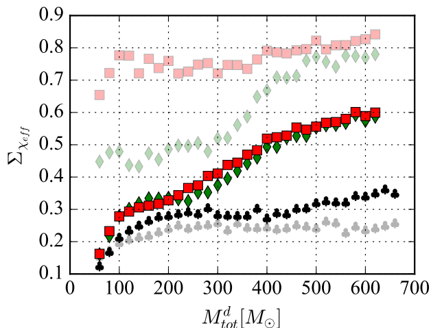
FIG. 22. 90% CI uncertainty in the effective spin along the orbital angular momentum against the detector frame total mass. The uncertainties in primary spin magnitude are also shown (semi-transparent symbols) for reference. See Table II for the parameters.
