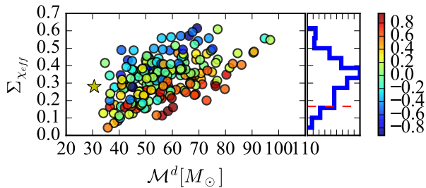
FIG. 14. The distribution of the 90% CI uncertainty in the estimation of \chi_{eff} (y axis) against the true detector-frame chirp mass (x axis). The colorbar shows the true \chi_{eff} . A star reports the coordinates of GW150914. The dashed line on the histogram marks the abscissa of the 10 th percentile.
