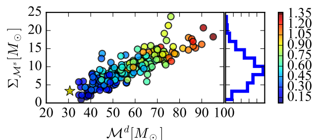
FIG. 4. The distribution of the 90% CI uncertainty in the estimation of the source-frame chirp mass (y axis) against the true detector-frame chirp mass (x axis). The colorbar is the redshift of the sources. A star reports the coordinates of GW150914.
