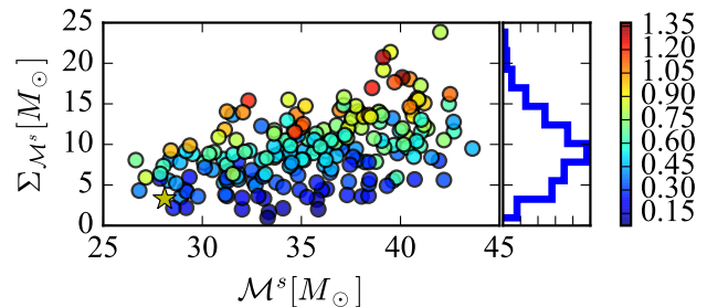
FIG. 3. The distribution of the 90% CI uncertainty in the estimation of the source-frame chirp mass (y axis) against the true source-frame chirp mass (x axis). The colorbar is the redshift of the sources. A star reports the coordinates of GW150914.
