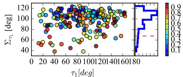
FIG. 17. The distribution of the 90% CI uncertainty in the estimation of the primary spin tilt angle (y axis, degs) against the true tilt angle (x axis, degrees). The colorbar shows the magnitude of the primary spin. The dashed line on the histogram marks the abscissa of the 10 th percentile.
