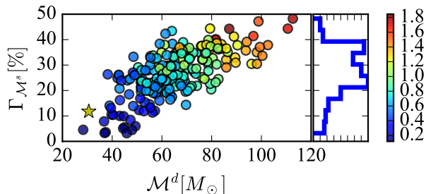
FIG. 26. For an HLVIJ network, the distribution of the 90% CI relative uncertainty (in percent over the true value) in the estimation of the source-frame chirp mass (y axis) against the true source-frame chirp mass (x axis). The colorbar is the redshift of the sources. A star reports the coordinates of GW150914.
