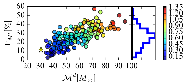
FIG. 8. The distribution of the 90% CI relative uncertainty (in percent over the true value) in the estimation of the source-frame total mass (y axis) against the true detector-frame chirp mass (x axis). The colorbar is the redshift of the sources. A star reports the coordinates of GW150914.
