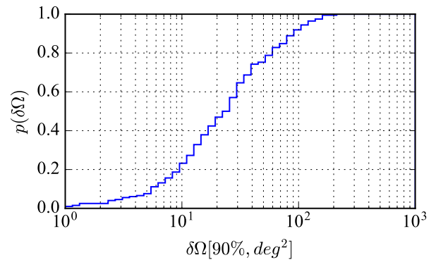
FIG. 28. Cumulative distribution for the 90% CI sky localization area for BBH detected by the HLVIJ network.
