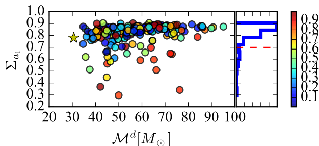
FIG. 9. The distribution of the 90% CI uncertainty in the estimation of the primary spin magnitude (y axis) against the true detector-frame chirp mass (x axis). The colorbar shows the magnitude of the primary spin. A star reports the coordinates of GW150914. The dashed line on the histogram marks the abscissa of the 10 th percentile.
