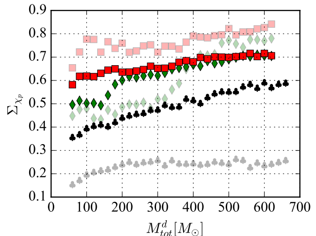
FIG. 23. 90% CI uncertainty in the effective spin along the plane of the orbit against the detector frame total mass. The uncertainties in primary spin magnitude are also shown (semi-transparent symbols) for reference. See Table II for the parameters.
