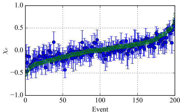
FIG. 15. For all events, median value of \chi_{eff} 90% CI. The empty green diamonds indicate the true values.
