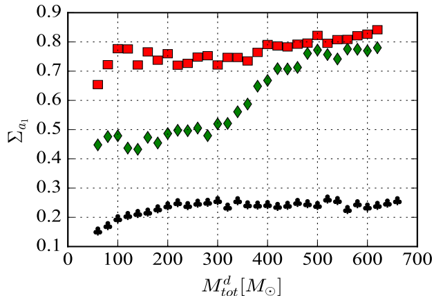
FIG. 21. 90% CI uncertainty in the primary spin magnitude against the detector frame total mass. See Table II for the parameters.
