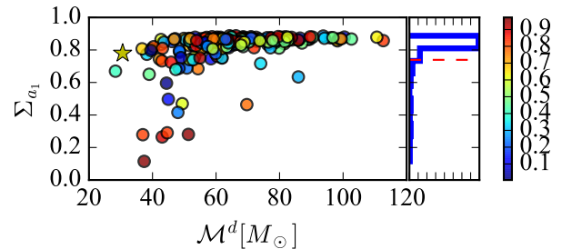
FIG. 27. For an HLVIJ network, the distribution of the 90% CI uncertainty in the estimation of the primary spin magnitude (y axis) against the true detector-frame chirp mass (x axis). The colorbar shows the magnitude of the primary spin. A star reports the coordinates of GW150914.
