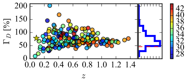
FIG. 18. The distribution of the 90% CI relative uncertainty (in percent over the true value) in the estimation of the luminosity distance (y axis) against the true redshift (x axis). The colorbar is the source-frame chirp mass of the sources, in M_{\odot} . A star reports the coordinates of GW150914. The dashed line on the histogram marks the abscissa of the 10 th percentile.
