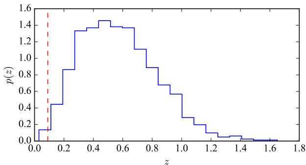
FIG. 1. The redshift distribution of detectable heavy BBH with a network of LIGO and Virgo at design sensitivity. The vertical dashed line is the median estimated redshift for GW150914 [4]
