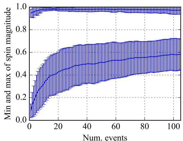
FIG. 25. The estimation of the minimum and maximum value of the spin magnitude for a population of BBH as more events are detected. The errorbars are obtained bootstrapping 100 sets of N events for each value of N , in the x axis. The true distribution is flat between 0.7 and 0.98. After 20 events, we can exclude non-spinning BBH in the underlying astrophysical population.
