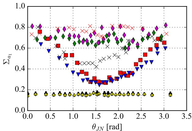
FIG. 20. 90% CI uncertainty in the primary spin magnitude against \theta_{JN} (rads) for various BBH sources. See Table I for the parameters of the sources.
