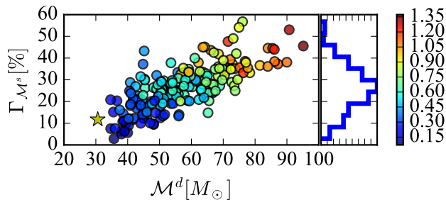
FIG. 5. The distribution of the 90% CI relative uncertainty (in percent over the true value) in the estimation of the source-frame chirp mass (y axis) against the true detector-frame chirp mass (x axis). The colorbar is the redshift of the sources. A star reports the coordinates of GW150914.
