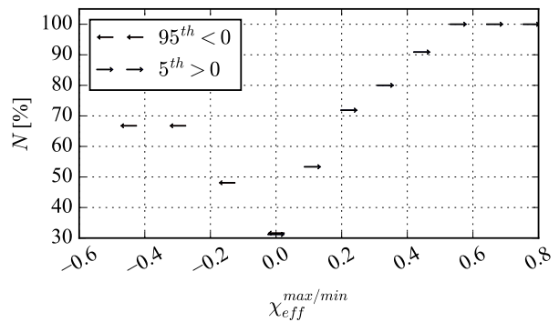
FIG. 16. The arrows pointing to the left report the fraction of events with true \chi_{eff} below that abscissa for which the 95 th percentile for \chi_{eff} is below zero. The arrows pointing to the right report the fraction of events with true \chi_{eff} above that abscissa for which the 5 th percentile for \chi_{eff} is above zero.
