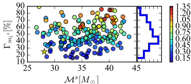
FIG. 6. The distribution of the 90% CI relative uncertainty (in percent over the true value) in the estimation of the source-frame primary mass (y axis) against the true source-frame chirp mass (x axis). The colorbar is the redshift of the sources. A star reports the coordinates of GW150914.
