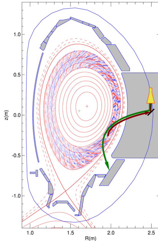
Figure 1. (Colour Online): Poloidal cross section of AUG with flux surfaces (for shot 22009) in red, with overlaid density fluctuation field from numerical simulations. The reflectometry antennas (at R = 2.407 m and z = 0.043 m) are shown to the right, with an emitted and a back-scattered ray.
