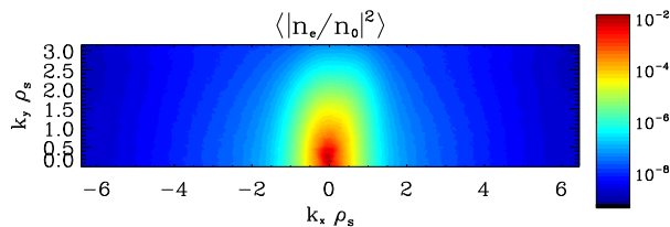
Figure 9. (Colour Online) Time-averaged electron density fluctuation spectrum from Sim 1 as function of the two wavenumbers perpendicular to the magnetic field line at (R, z) = (2.01, -0.175) m.
