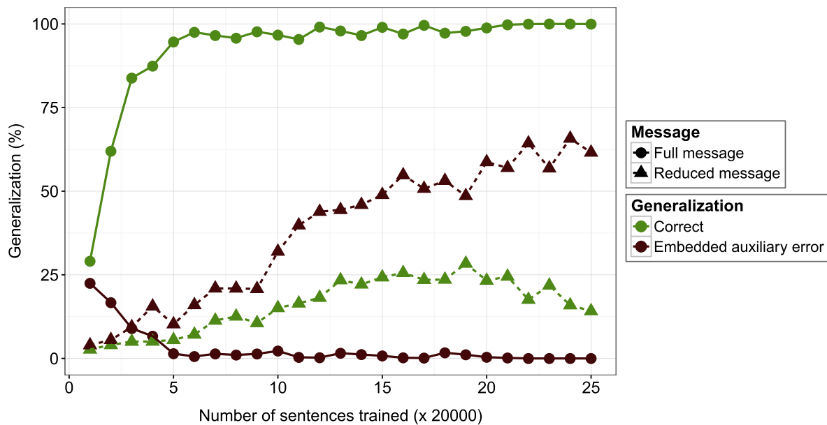
Fig. 6. Different generalization abilities in the model when the influence of sentence meaning was reduced in the EVENT SEMANTICS, compared with a full message.
