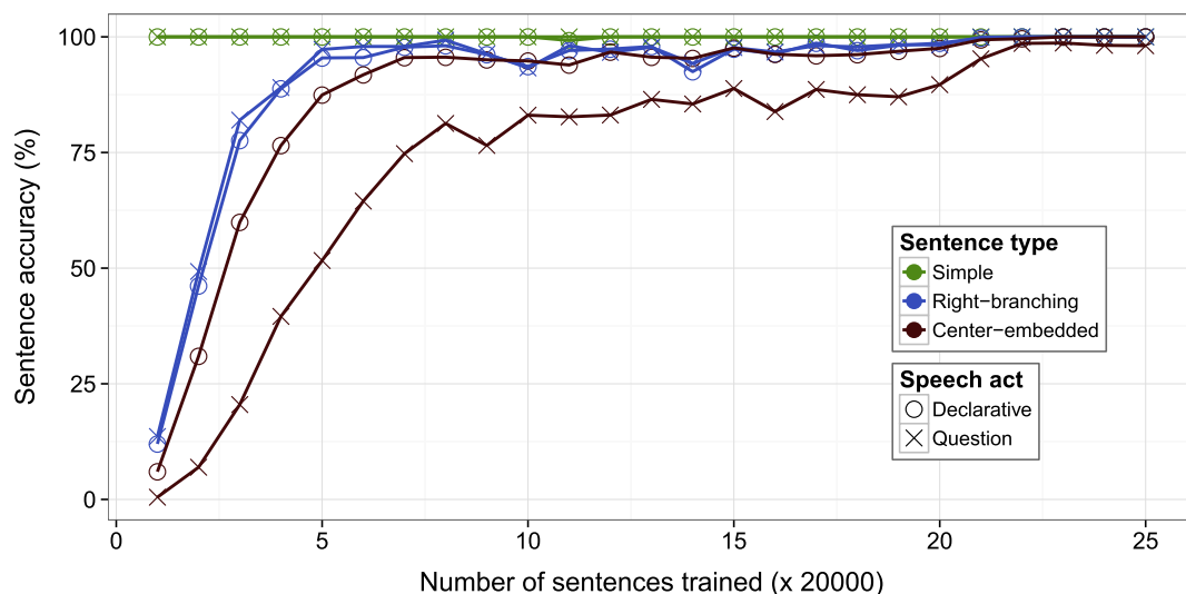
Fig. 3. Model performance for all structural types in the input language, which were either single-clause, right-branching or center-embedded questions and declaratives. Center-embedded questions were novel polar questions with two auxiliaries which were not present in the model's learning environment.
