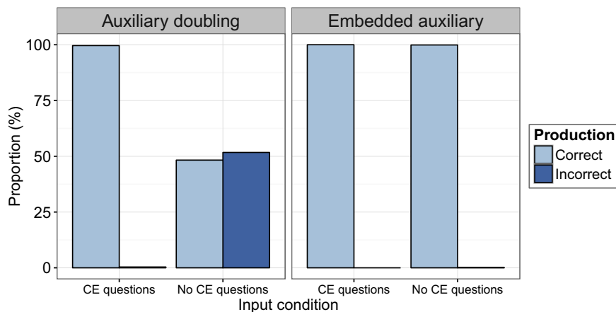
Fig. 8. Model performance with and without center-embedded yes-no questions with a main clause auxiliary in the input, averaged over the final three test points. Neither input condition contained center-embedded questions with two auxiliaries.
