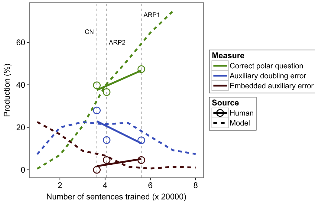
Fig. 5. Error comparison between the model and child production data from three age groups over development. CN denotes the weighted average of Experiments 1 and 2 in Crain and Nakayama (1987), ARP1 and ARP2 refer to Experiments 1 and 2, respectively, in Ambridge et al. (2008).
