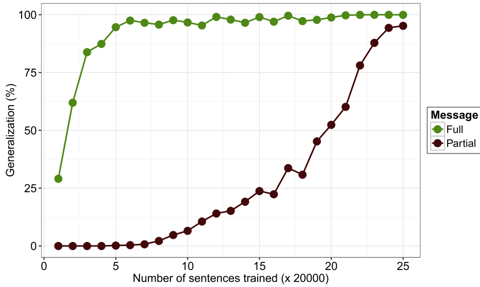
Fig. 7. Structure-dependent generalization when messages were developing over time, compared with a model where full messages were available from the beginning of acquisition.
