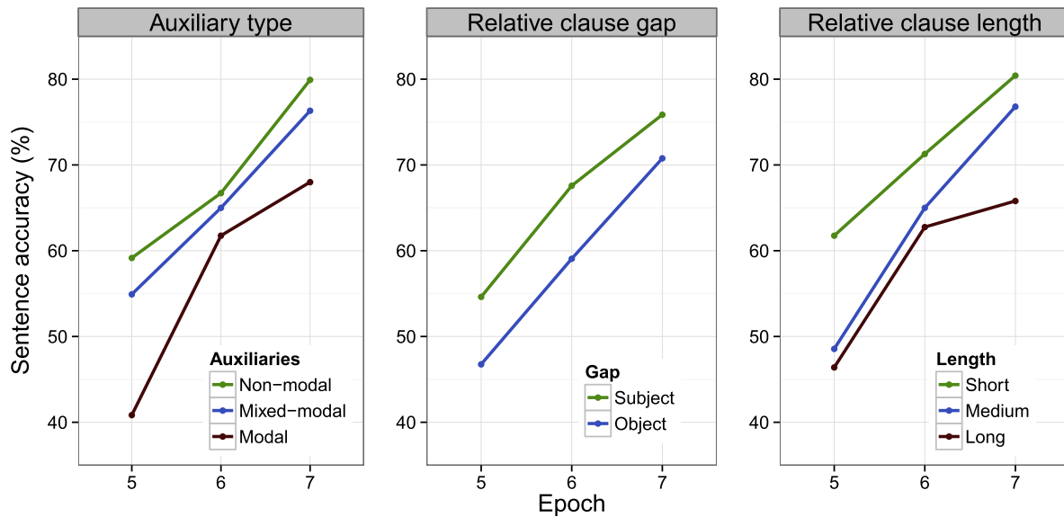
Fig. 4. Cross-section of production accuracy on complex questions distinguished by auxiliary type in the main and embedded clause (modal, non-modal, mixed-modal), relative clause type (subject, object gap), and relative clause length (short, medium, long).
