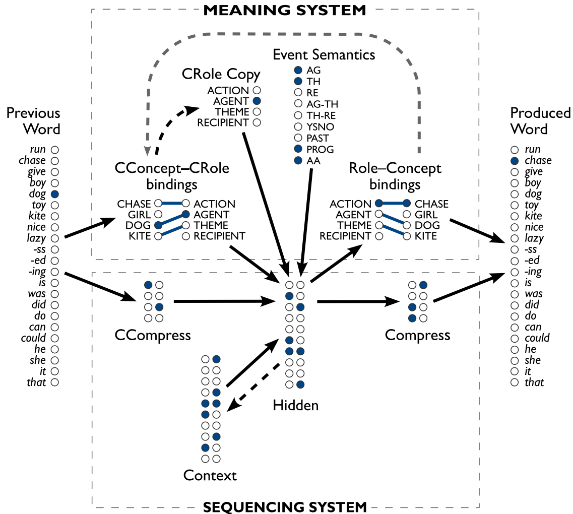
Fig. 2. Architecture of the Dual-path model (Chang et al., 2006). Word input arrived at the PREVIOUS WORD layer and activation spread through the sequencing and meaning pathways to the PRODUCED WORD output layer. The sequencing system represented word categories at the CCOMPRESS and COMPRESS layers and learned abstract syntactic frames over these categories. The meaning system represented a sentence-specific message that the model learned to activate incrementally at the right point in time. The two pathways intersected at the HIDDEN layer and competed/cooperated at the output layer. Solid arrows indicate connection weights that were adapted during learning, fixed copy connections are represented by dashed arrows. Solid links between roles and concepts in the respective layers were set during production and enabled binding. The conceptual structure of the target utterance was represented by features in the EVENT SEMANTICS layer which also signaled the intended speech act.
