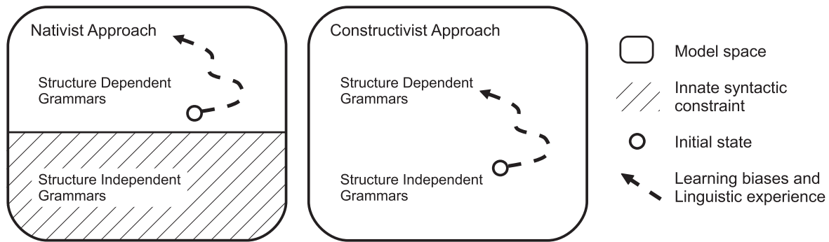
Fig. 1. Schematic of nativist and constructivist accounts of auxiliary inversion.
