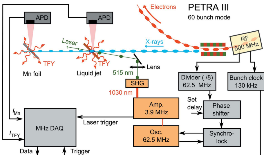
Figure 2 Sketch of the experimental setup at the dynamics beamline P01 of PETRA III (here: in 60-bunch mode delivering X-ray pulses at 7.8 MHz), including a fiber amplifier laser system synchronized to the RF frequency of the storage ring and our MHz DAQ system capable of digitizing and integrating the APD detector signal traces.
