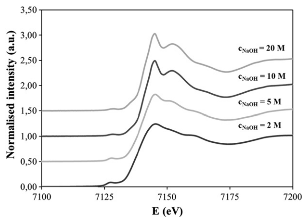
Fig. 6. Fe–K-edge XANES spectra of the solid substances obtained from solutions with varying concentrations of NaOH.
