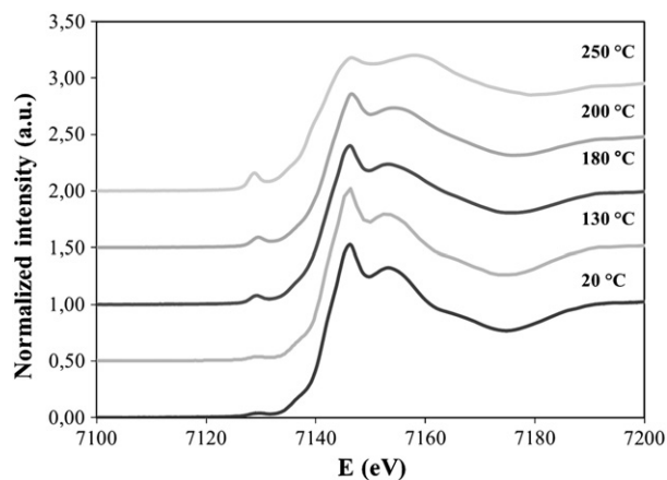
Fig. 7. Fe–K-edge X-ray absorption spectra on BaFe-LDH-10 samples after calcination at various temperatures.
