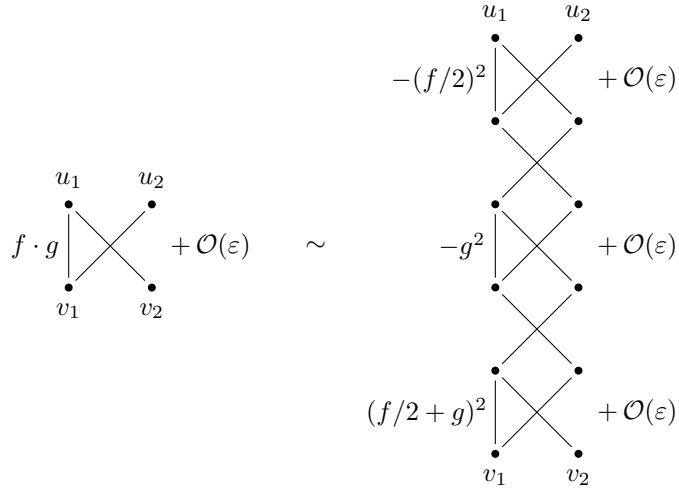
Figure 4: Multiplication construction for Lemma 3.4
