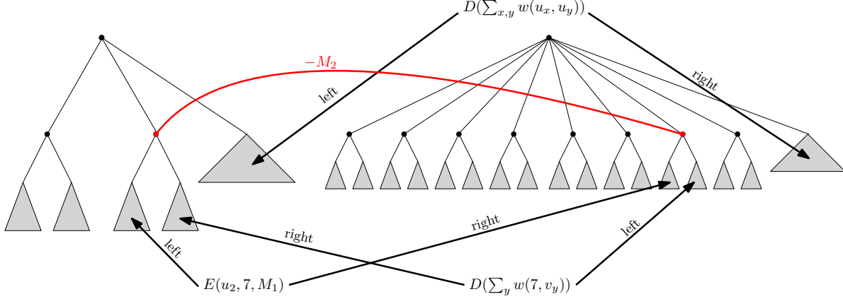
Figure 6: Schematic illustration of a connection gadget for k/3 = 2 and n = 8 .
