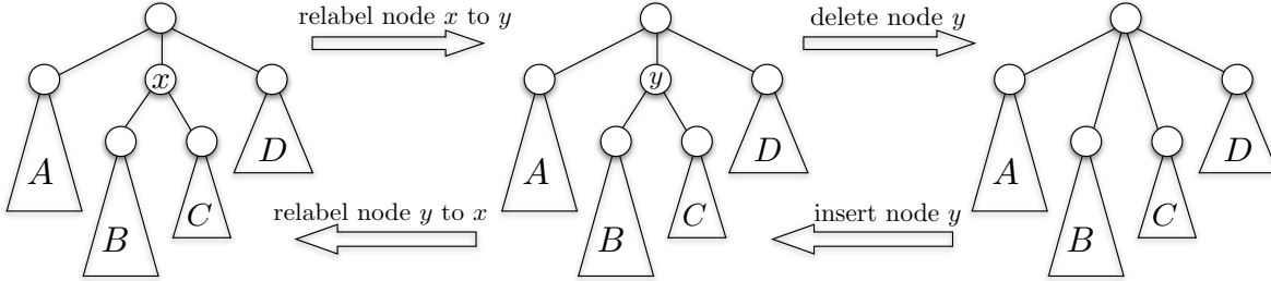
Figure 1: The three editing operations on a tree with vertex labels.
