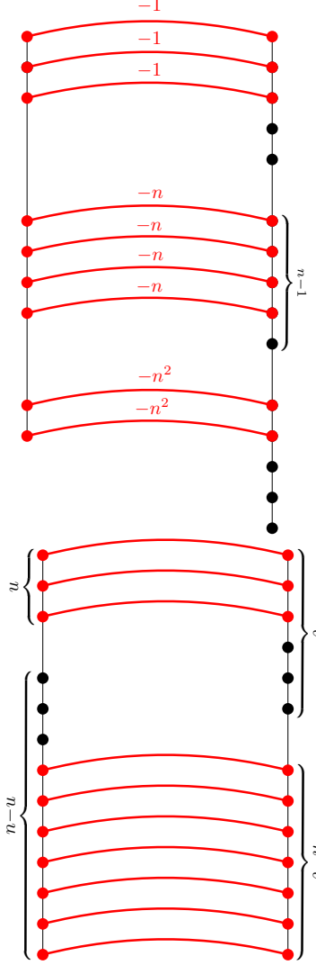
Figure 5: Left: Decrease gadget built for d = 3 , n = 6 and x = n^2 \cdot 2 + n \cdot 4 + 3 . Right: Equality gadget for u = 3 , v = 6 .
