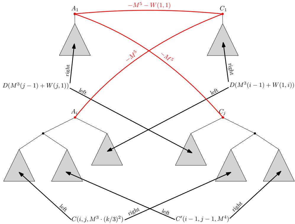
Figure 7: Micro structures A_1, C_1 and A_i, C_j for i, j > 1 .
