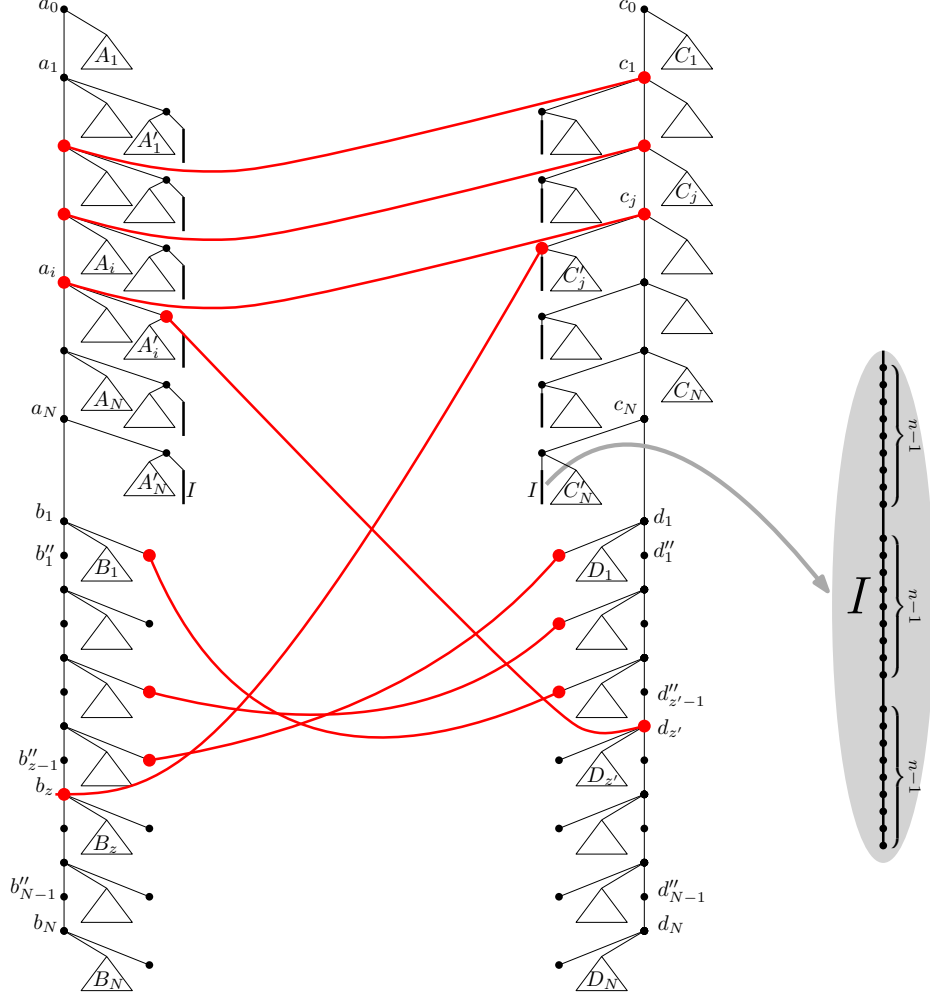
Figure 4: A hard instance of TED constructed for a given instance of max-weight k -clique.
