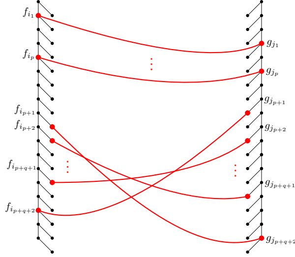
Figure 2: Macro structure of the hard instance for TED: A tree F composed of a single spine with leaves hanging to the right and a tree G composed of a single spine with leaves hanging to the left.
