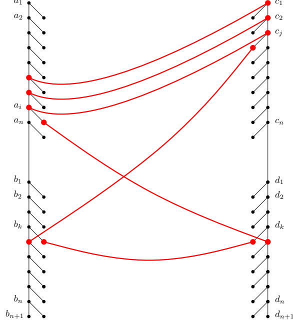
Figure 3: A hard instance of TED constructed for a given instance of negative triangle detection. Appropriately chosen costs ensure that any optimal solution has a specific structure.
