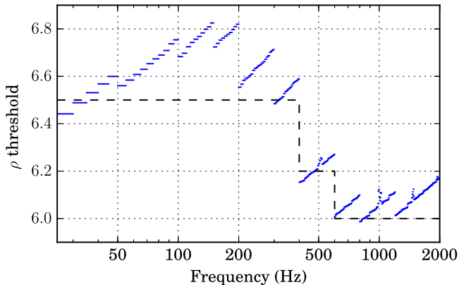
Figure 3. Selection of follow-up threshold as a function of frequency. If the data contained no signal and only Gaussian noise, each template in parameter space would have some chance of producing a statistic value exceeding a given threshold. Within each 0.05 Hz frequency band, the total number of templates was computed and used to find the threshold at which the expected number of Gaussian outliers above that value would be 0.1 (short blue lines). For simplicity, the actual follow-up threshold was chosen near or below that level, producing thresholds of 6.5 for 25 \text{ Hz} < f_0 < 400 \text{ Hz} , 6.2 for 400 \text{ Hz} < f_0 < 600 \text{ Hz} , and 6.0 for 600 \text{ Hz} < f_0 < 2000 \text{ Hz} (black dashed line). Note that the large number of non-Gaussian outliers (cf. Table 3) makes the Gaussian follow-up level an imprecise tool in any event.
