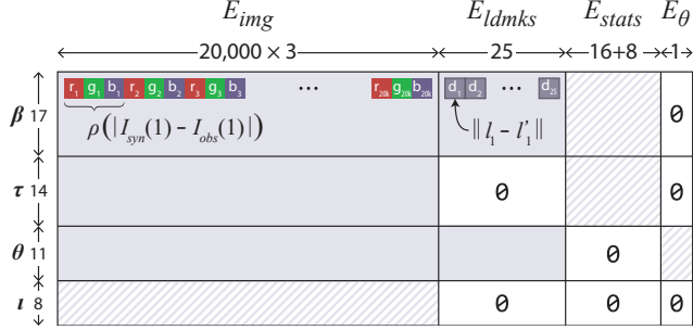
Figure 8. The non-zero structure of our Jacobian \mathbf{J}_r for a 200 \times 100 px eye region. \mathbf{J}_r is calculated entirely on the GPU. Dashed regions represent sparse blocks.
