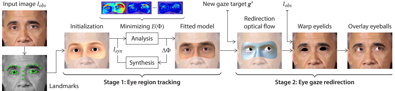
Figure 3. Given observed image I_{obs} , we first initialize our model using 25 facial landmarks from a face tracker [1]. We then find optimal model parameters \Phi^* using analysis-by-synthesis, minimizing a reconstruction energy E(\Phi) . We then modify \Phi^* with the desired gaze and eyelid behaviour, resulting in a new I_{syn} which we blend onto I_{obs} , giving a redirected gaze image.
