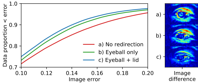
Figure 13. Redirection error decreases as we enable more parts of our redirection pipeline. The x -axis represents image error, and the y -axis represents the proportion of data under that error.
