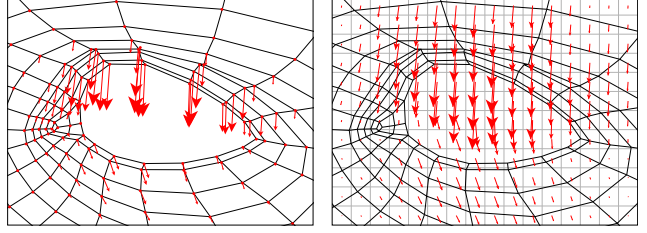
Figure 9. We efficiently convert sparse per-vertex image-space flows (left) to a dense per-pixel flow field (right) using GPU rasterization. We use this dense flow-field to warp the eyelids.
