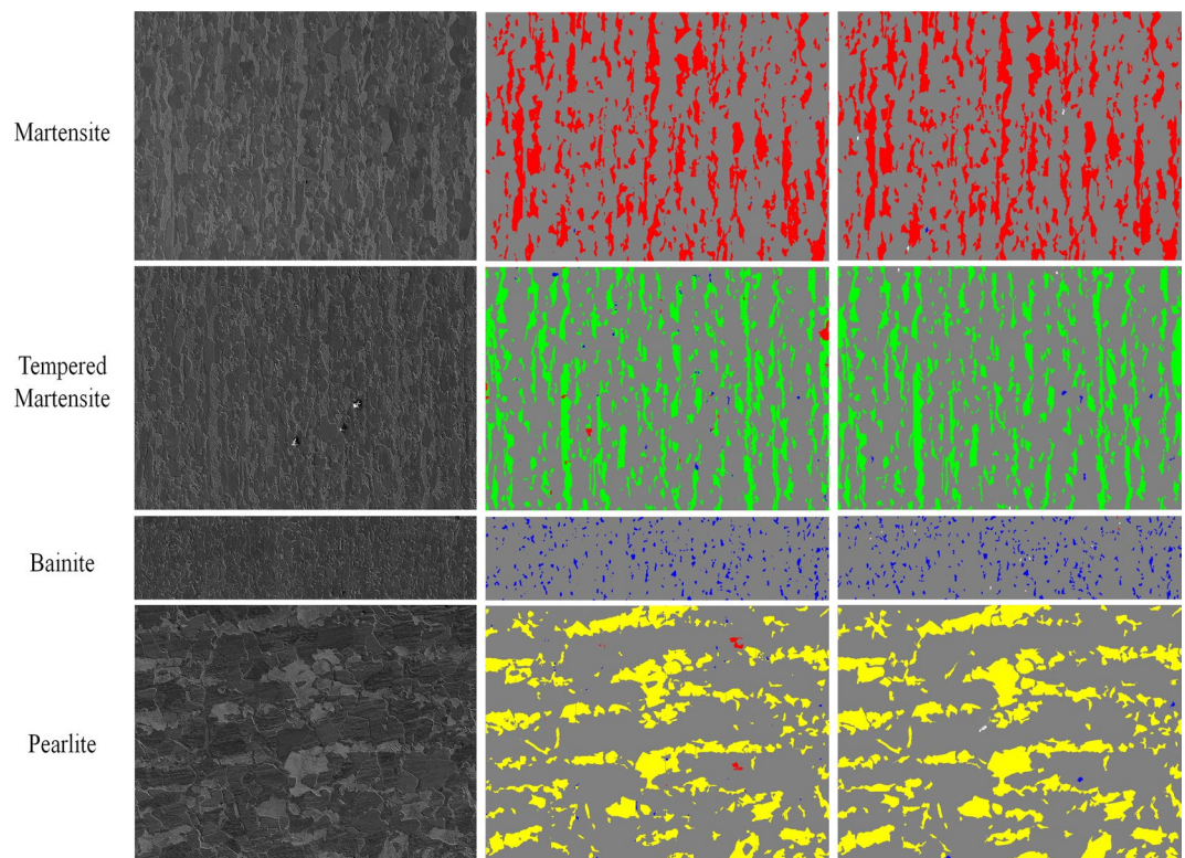
Figure 7. Examples of applying a max-voting scheme to stitched and segmented SEM patches for different microstructure classes. The ground truth colors of martensite, tempered martensite, bainite and pearlite are red, green, blue, and yellow, respectively. Not-segmented objects in the segmentation phase are shown with white color.
