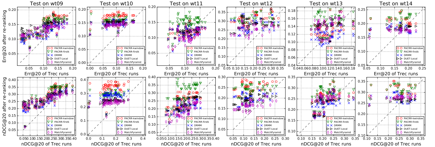
Figure 3: Re-ranking search results from Trec Web Track 2009–14 runs with PACRR-kwindow, PACRR-firstsk, DRMM, Duet-local and MatchPyramid respectively. The x-axis represents the ranking score of the original TREC runs and the y-axis represents the score of the corresponding re-ranked runs. The dashed line is y=x . Err@20 is used in the upper row and nDCG@20 is used in the lower row.
