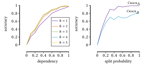
Fig. 4. [Higher is better] Accuracy of CRACK on synthetic data of different tree heights (left) and with different split probabilities (right).
