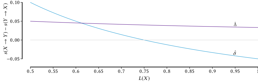
Fig. 1. Effect of the domain size of X on \hat{\Delta} and \hat{\delta} by keeping L(Y) and the gains in compression constant. If s(X \rightarrow Y) - s(Y \rightarrow X) of the corresponding score is < 0 it infers X \rightarrow Y and for > 0 it infers Y \rightarrow X .
