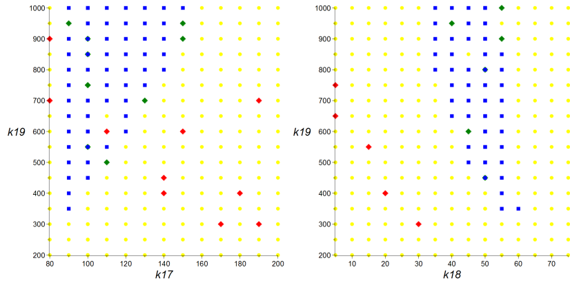
Fig. 2. Bertini grid sampling on the original version of Biomod-26 (see Sect. 4.1)
