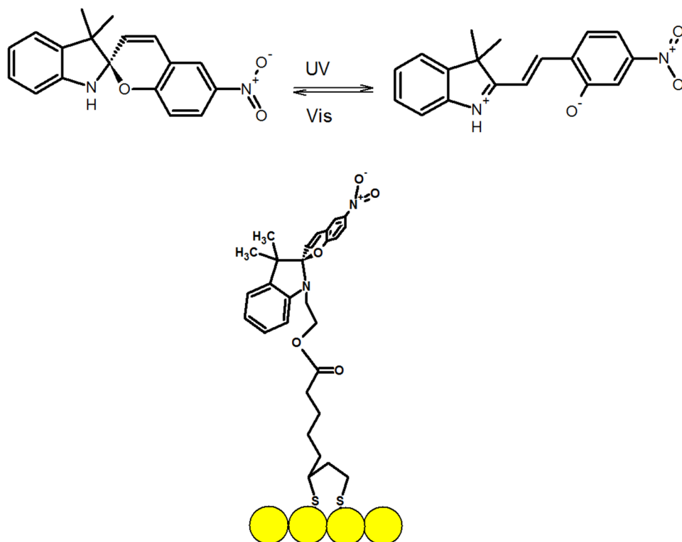
Figure 1. Interconversion between the closed SP—and the open MC-form under irradiation with light for a 6-Nitro-BIPS unit. Below 2-(3'3'-Dimethyl-6-nitro-3' H -spiro[chromene-2,2'-indol]-1'-yl)ethyl(1,2-dithiolane-3)pentanoate (SP-LA) attached on a gold surface as used in this study.
