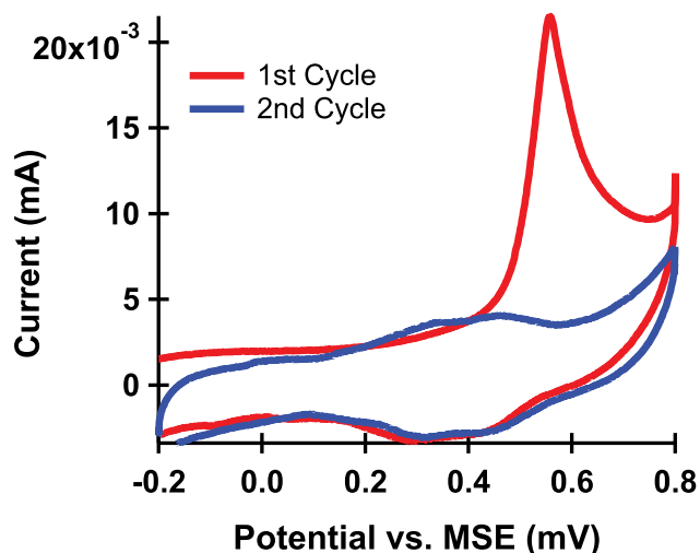
Figure 4. Cyclic voltammogram of our SP-LA SAM on a gold electrode versus an MSE reference at a 50 \text{ mV s}^{-1} scan rate. In the first run at +0.56 \text{ V} an irreversible oxidation takes place leading to a new species at the surface that shows reversible redox behavior in the second and all further scans.
