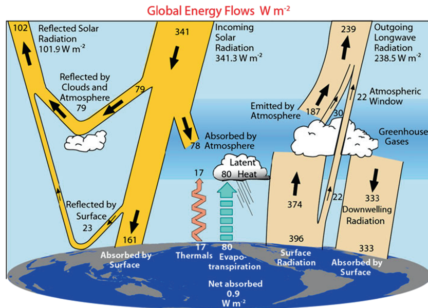
Figure 6. Global annual mean Earth’s energy budget for 2000–2005 ( W m^{-2} ). Reprinted with permission from Trenberth and Fasullo [2012].
