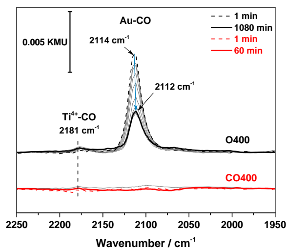
Figure 5: Sequence of DRIFT spectra in the CO ad region, recorded during CO adsorption (1% CO, 99% N 2 ) at 80 °C on a Au/TiO 2 catalyst, pretreated at 400 °C in oxidizing (O400, 10% O 2 / 90% N 2 ) or reducing (CO400, 10% CO / 90% N 2 ) atmospheres.
