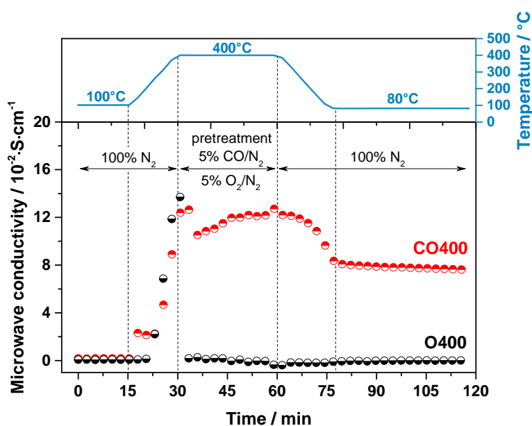
Figure 6: Microwave conductivity of Au/TiO 2 before, during and after pretreatment at 400 °C in oxidizing (O400: 5% O 2 / 95% N 2 ) or reducing (CO400: 5% CO / 95% N 2 ) atmosphere.
