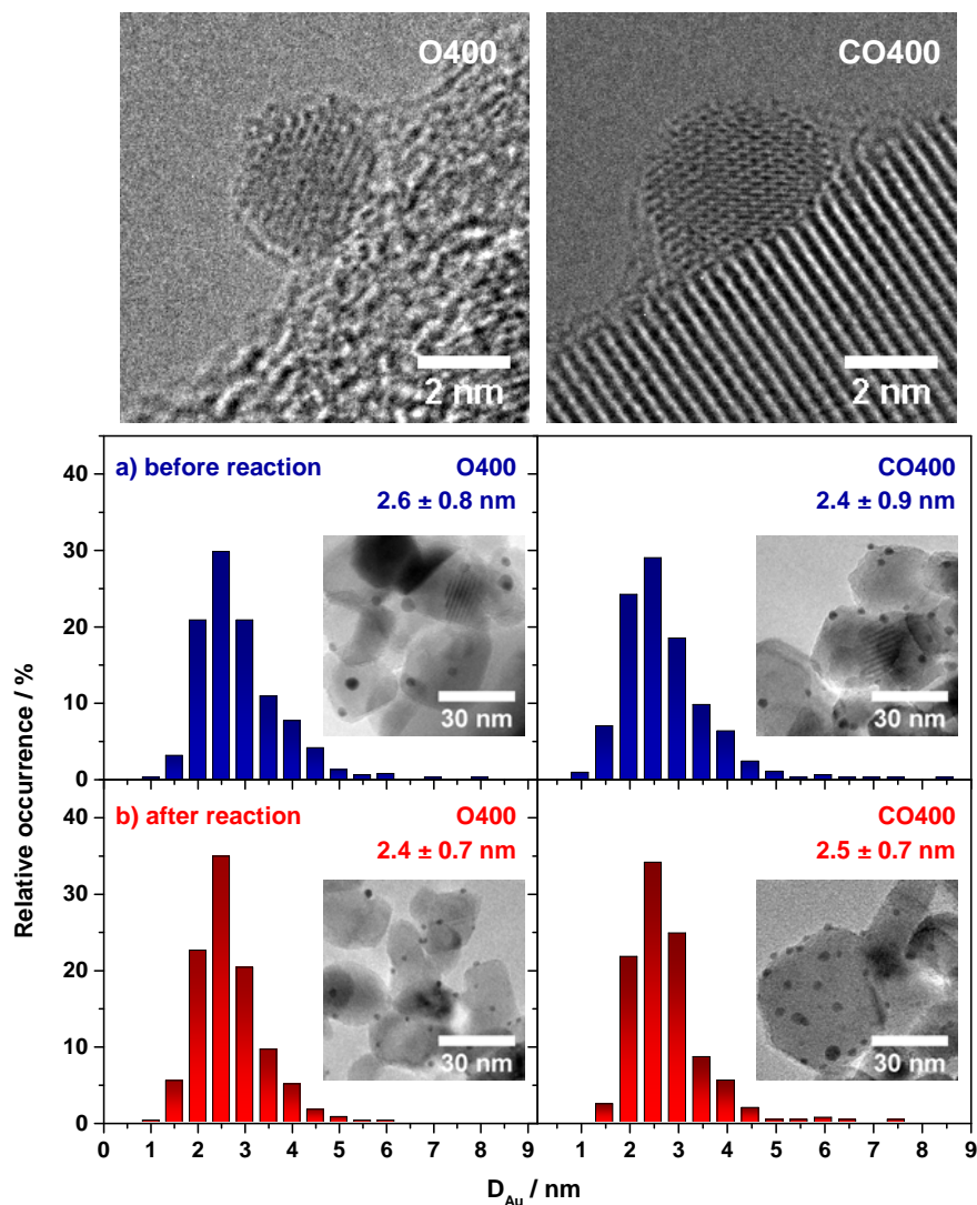
Figure 1: Au particle size distributions and representative high resolution and overview TEM images of the Au/TiO 2 catalyst pretreated at 400 °C in oxidizing (O400, 10% O 2 / 90% N 2 ) or reducing (CO400, 10% CO / 90% N 2 ) atmosphere (a) before and (b) after CO oxidation at 80 °C for 1000 min.
