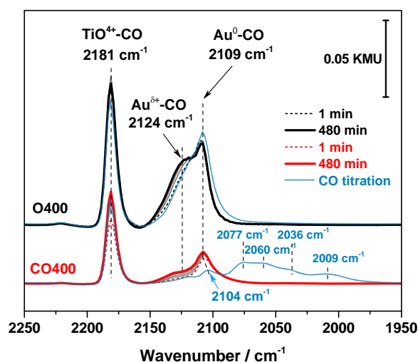
Figure 11: Sequence of DRIFT spectra representing adsorbed CO species (CO ad ), recorded during CO oxidation (1% CO, 1% O 2 , 98% N 2 ) and CO adsorption (1% CO, balance N 2 ) at -20 °C on Au/TiO 2 catalysts pretreated at 400 °C in oxidizing (O400, 10% O 2 / 90% N 2 ) or reducing (CO400, 10% CO / 90% N 2 ) atmosphere. Note that the gas phase CO signal is already subtracted.
