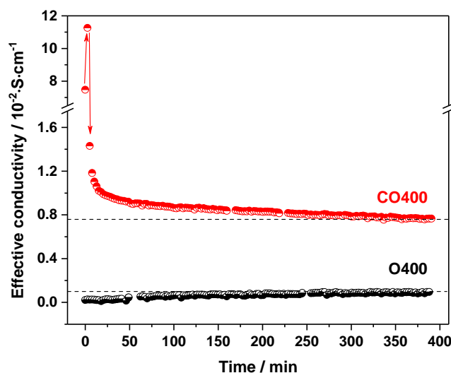
Figure 7: Microwave conductivity of Au/TiO 2 during the CO oxidation (1% CO, 1% O 2 , 98% N 2 ) at 80 °C after pretreatment in oxidizing (O400: 5% O 2 / 95% N 2 ) or reducing (CO400: 5% CO / 95% N 2 ) atmosphere, respectively.
