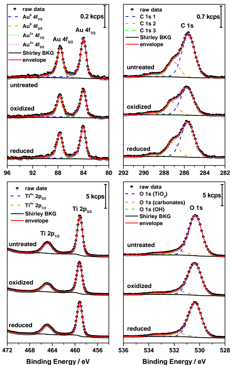
Figure 2: XP spectra of the Au 4f, C 1s, Ti 2p, and O 1s signals obtained on Au/TiO 2 catalysts as received (untreated) and after oxidizing (O400, 10% O 2 / 90% N 2 ) or reducing (CO400, 10% CO / 90% N 2 ) pretreatment.
