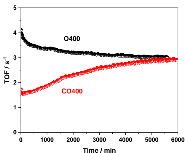
Figure 3: Turn over frequencies (TOFs) for CO oxidation (1% CO, 1% O 2 , 98% N 2 ) on Au/TiO 2 at 80 °C after in situ pretreatment at 400 °C in oxidizing (O400: 10% O 2 / 90% N 2 ) or reducing (CO400: 10% CO / 90% N 2 ) atmosphere.
