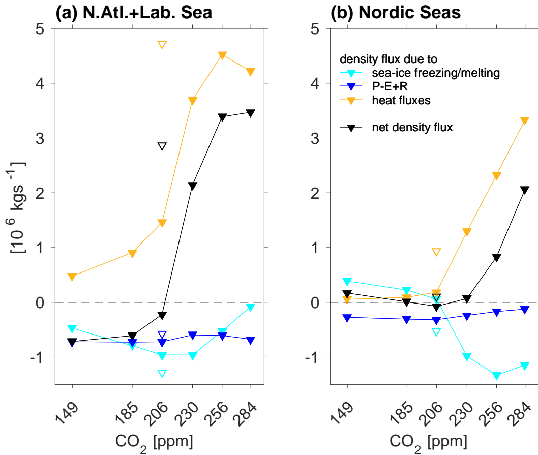
Figure 5.3: Annual mean net density flux (black) as a function of pCO_2 , and its components: density flux due to heat loss or gain (orange), due to atmospheric fresh-water input (blue) and due to sea-ice freezing and melting (cyan). The fluxes are integrated over the OOC_{max} region of (a) the North Atlantic including the Labrador Sea, and (b) the Nordic Seas. Positive values indicate a density gain, negative values indicate a density loss. The open symbols indicate the pi206_s composite. The x-axis is scaled logarithmically.
