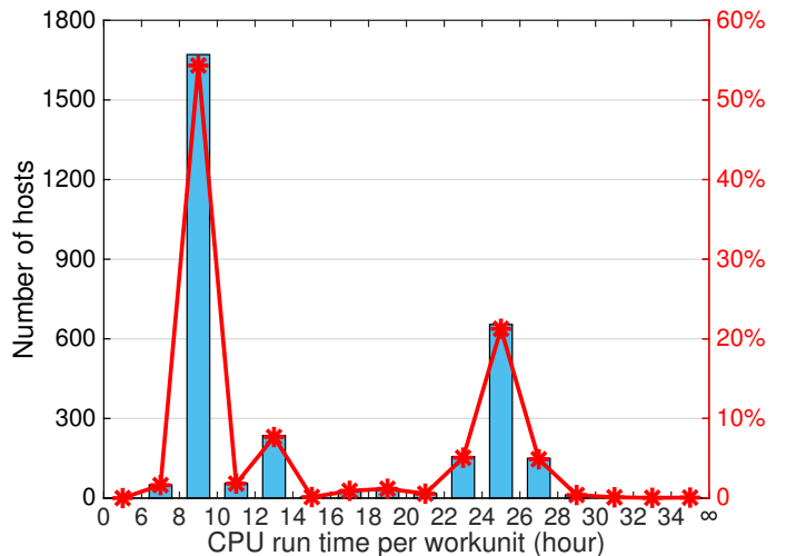
FIG. 2: Distribution of the run-times of the Einstein@Home O1 low frequency all-sky search WUs. The data in this figure is taken from a sample of 3076 hosts out of total 28764 hosts of Einstein@Home.
