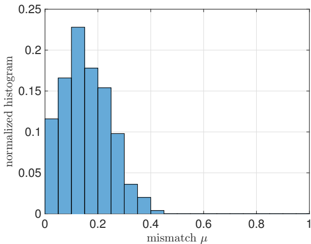
FIG. 1: This histogram shows the mismatch distribution for the grid spacing: m_f = 0.15 , m_j = 0.3 , m_{\dot{f}} = 0.003 , \gamma^{(1)} = 8 , \gamma^{(2)} = 20 and T_{\text{coh}} = 15 days. The average measured mismatch is \langle \mu \rangle = 15.8\% .
