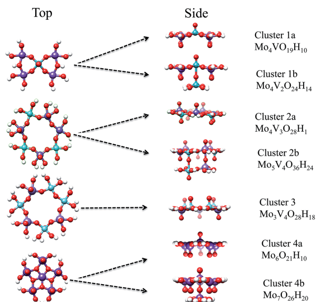
Fig. 5 Top and side view of the hydrogen saturated cluster models used to model the MoV topologies of the MoVO x catalyst. In particular, mono-layered clusters 1a: Mo 4 V 19 H 10 , 2a: Mo 4 V 3 O 28 H 18 , 3: Mo 3 V 4 O 28 H 18 and 4a: Mo 6 O 21 H 10 as well as bilayer 1b: Mo 4 V 2 O 24 H 14 , 2b: Mo 5 V 4 O 36 H 24 and 4b: Mo 7 O 26 H 20 are visualized (color coding: Mo, purple, V, cyan, O, red, H, white).
