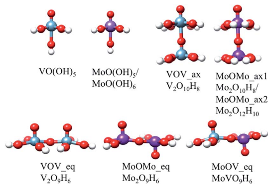
Fig. 4 Monomeric and dimeric model structures of VO(OH) 5 , MoO(OH) 5 , VOV_ax: V 2 O 10 H 8 , VOV_eq: V 2 O 9 H 6 , MoOMo_ax: Mo 2 O 10 H 8 , MoOMo_eq: Mo 2 O 9 H 6 and MoOV_eq: MoVO 9 H 6 (color coding: Mo, purple, V, cyan, O, red, H, white).
