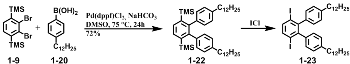
Abbildung 70: Syntheseroute zu Diiod-Dodecyl- o -terphenyl 1-23
