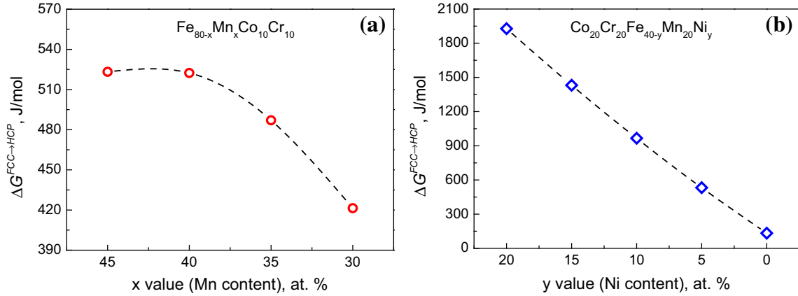
Fig. 2. Free energy differences ( \Delta G ) between the FCC and HCP structures of typical alloy systems at 300 K derived by thermodynamic calculations using the Calphad approach (Thermo-Calc, database TCFE7): (a) quaternary \text{Fe}_{80-x}\text{Mn}_x\text{Co}_{10}\text{Cr}_{10} ( x = 45 at.%, 40 at.%, 35 at.%, and 30 at.%) and (b) quinary \text{Co}_{20}\text{Cr}_{20}\text{Fe}_{40-y}\text{Mn}_{20}\text{Ni}_y ( y = 20 at.%, 15 at.%, 10, 5 at.%, and 0 at.%).
