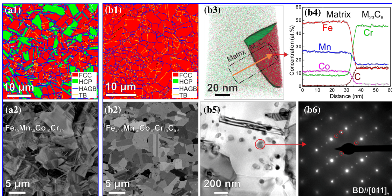
Fig. 5. Typical microstructures of \text{Fe}_{50}\text{Mn}_{30}\text{Co}_{10}\text{Cr}_{10} and \text{Fe}_{49.5}\text{Mn}_{30}\text{Co}_{10}\text{Cr}_{10}\text{C}_{0.5} alloys after recrystallization annealing for 3 min: (a 1 ) EBSD phase map and (a 2 ) ECC image of dual-phase \text{Fe}_{50}\text{Mn}_{30}\text{Co}_{10}\text{Cr}_{10} alloy; (b 1 ) EBSD phase map, (b 2 ) ECC image, (b 3 ) APT tip reconstruction, (b 4 ) elemental profiles across an interface of matrix and carbide, (b 5 ) TEM bright-field image, and (b 6 ) selected-area diffraction pattern of interstitial \text{Fe}_{49.5}\text{Mn}_{30}\text{Co}_{10}\text{Cr}_{10}\text{C}_{0.5} alloy. Diffraction spots marked by red circles in (b 6 ) show the FCC structure of the \text{M}_{23}\text{C}_6 carbides (Color figure online).
