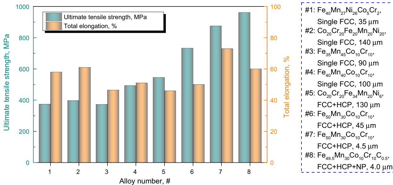
Fig. 6. Overview of ultimate tensile strength and total engineering elongation obtained for various non-equiatom high-entropy alloys. For comparison, data of the equiatomic \text{Co}_{20}\text{Cr}_{20}\text{Fe}_{20}\text{Mn}_{20}\text{Ni}_{20} alloy (#2) are also shown. All alloys produced in-house using similar processing routes shown in Fig. 2 for full control of the experimental setup. All these data stem from uniaxial tensile tests conducted on bulk samples with identical dimensions at room temperature at strain rate of 1 \times 10^{-3} \text{ s}^{-1} .
