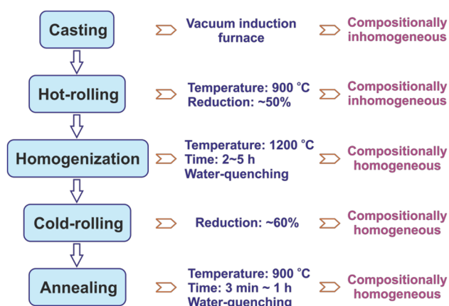
Fig. 3. Processing routes and related parameters as well as resultant compositional homogeneity states for 3d transition-metal high-entropy alloys.
