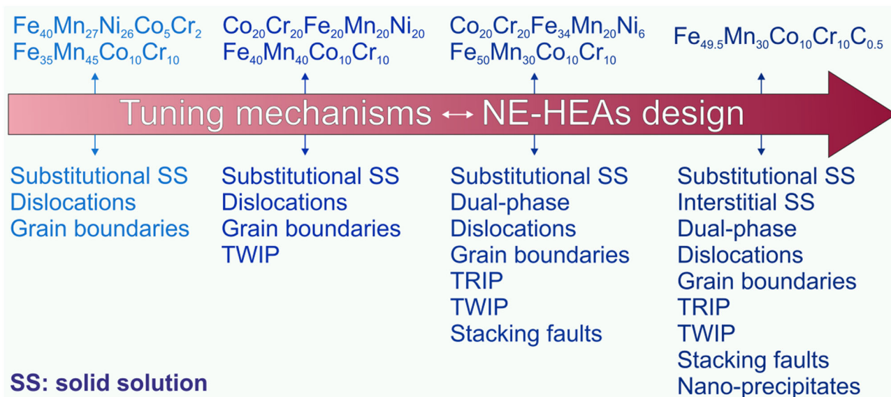
Fig. 7. Overview of deformation mechanisms in various multicomponent high-entropy alloys showing that tuning deformation mechanisms is key to development of strong and ductile non-equiatomic high-entropy alloys (NE-HEAs). The strength and ductility of these alloys are given in Fig. 6. SS: solid solution.
