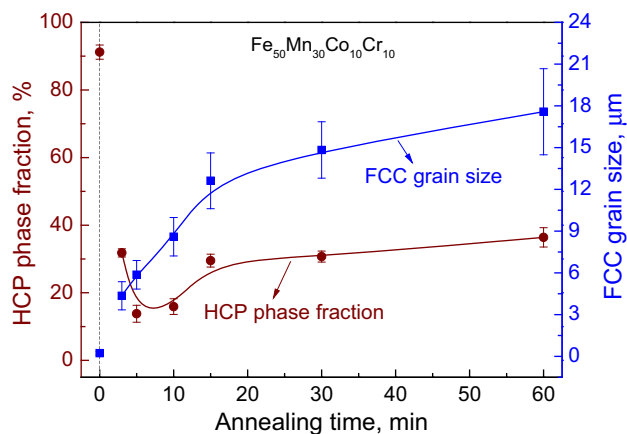
Fig. 4. Variations in FCC grain size and HCP phase fraction in dual-phase \text{Fe}_{50}\text{Mn}_{30}\text{Co}_{10}\text{Cr}_{10} alloy with increasing annealing time at 900^\circ\text{C} . Annealing time of 0 min refers to the cold-rolled state of the samples without annealing. Data mainly taken from Ref. 13.
