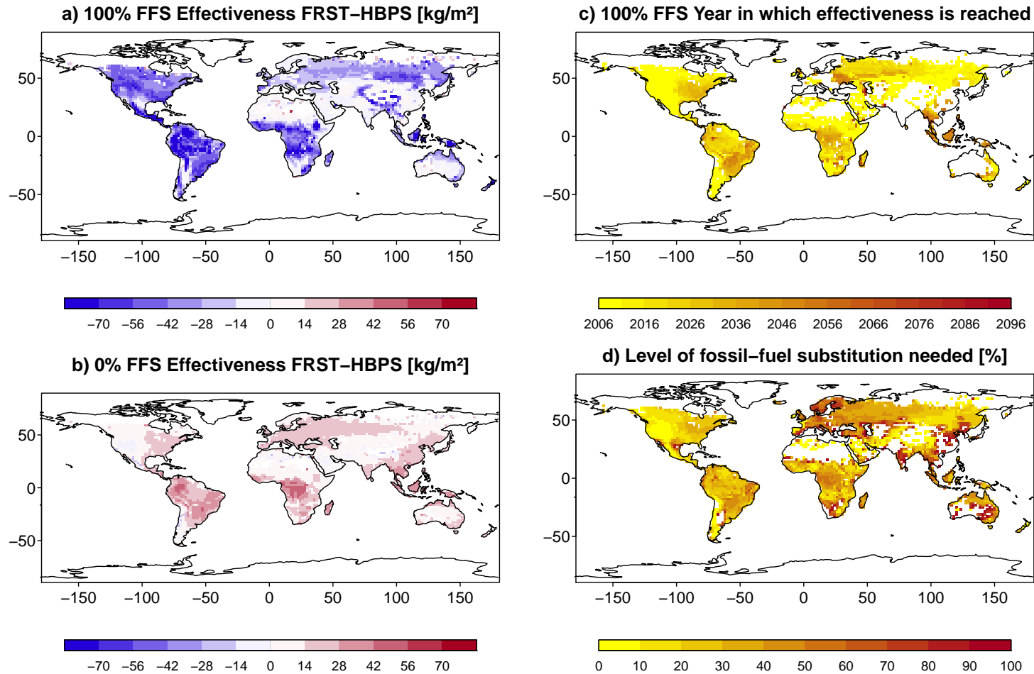
Figure 3.9: Effectiveness of herbaceous biomass plantations compared to forests: a) for 100% fossil-fuel substitution, b) for 0% fossil-fuel substitution. c) Year in which 5-year mean effectiveness becomes negative in each gridcell for 100% fossil-fuel substitution. d) Level of fossil-fuel substitution needed for herbaceous biomass plantations to exceed the effectiveness of forests in the year 2100. All graphs refer to the simulations with 71% harvest (HBPs71). FFS: fossil-fuel substitution, FRST-HBPS: measure of effectiveness, carbon density of forests minus carbon density of herbaceous biomass plantations (including fossil-fuel substitution for the lifetime of the plantations).
