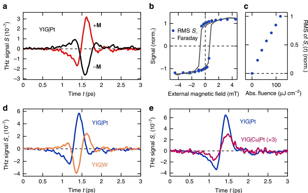
Fig. 2 Terahertz emission of photoexcited F/N bilayers. a THz emission signals S(\pm\mathbf{M}) from a YIG(3 \mu\text{m} )|Pt(5.5 nm) sample for opposite directions of the in-plane YIG magnetization \mathbf{M} as a function of time t . We focus on the difference S_- = S(\mathbf{M}) - S(-\mathbf{M}) odd in \mathbf{M} . b Amplitude of the THz signal S_- (root-mean-square, RMS) and the Faraday rotation of a continuous-wave laser beam (wavelength 532 nm) as a function of the external magnetic field. Both hysteresis loops were measured under identical pump conditions at room temperature. c Amplitude of S_- as a function of the absorbed pump fluence. d THz emission signal from a 3 \mu\text{m} thick YIG film capped with Pt and W, both 5.5 nm thick. e THz emission signal from a 5 \mu\text{m} YIG film capped with Pt(5.6 nm) or Cu(1.9 nm)|Pt(5.4 nm)
