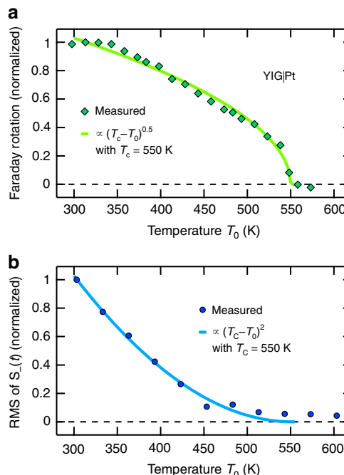
Fig. 3 Effect of sample temperature. a Faraday rotation of a continuous-wave laser beam (wavelength 532 nm) after transmission through a YIG(3 \mu\text{m} )|Pt(5.5 nm) sample as a function of the sample temperature. A fit proportional to (T_C - T_0)^\alpha (ref. 33) yields a critical exponent of \alpha = 0.5 and a Curie temperature of T_C = 550 K. b Temperature dependence of the amplitude of the magnetic THz emission signal S_- , which differs from that of the sample magnetization, similar to previous work on the DC SSE 32 . The solid line is a fit proportional to (T_C - T_0)^\alpha , here yielding \alpha = 2.0 \pm 0.5
