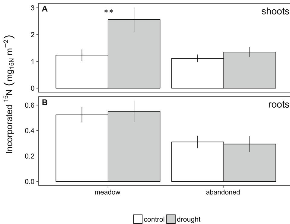
Figure 5. Amount of 15 N label recovered in the two grasslands in A shoots and B roots of control monoliths ( open bars ) and in monoliths recovering from drought ( shaded bars ) 3 weeks after the rewetting. Error bars indicate standard errors of the mean ( n = 3). Stars indicate significant differences between control and drought treatment ( p value: ** < 0.01).
