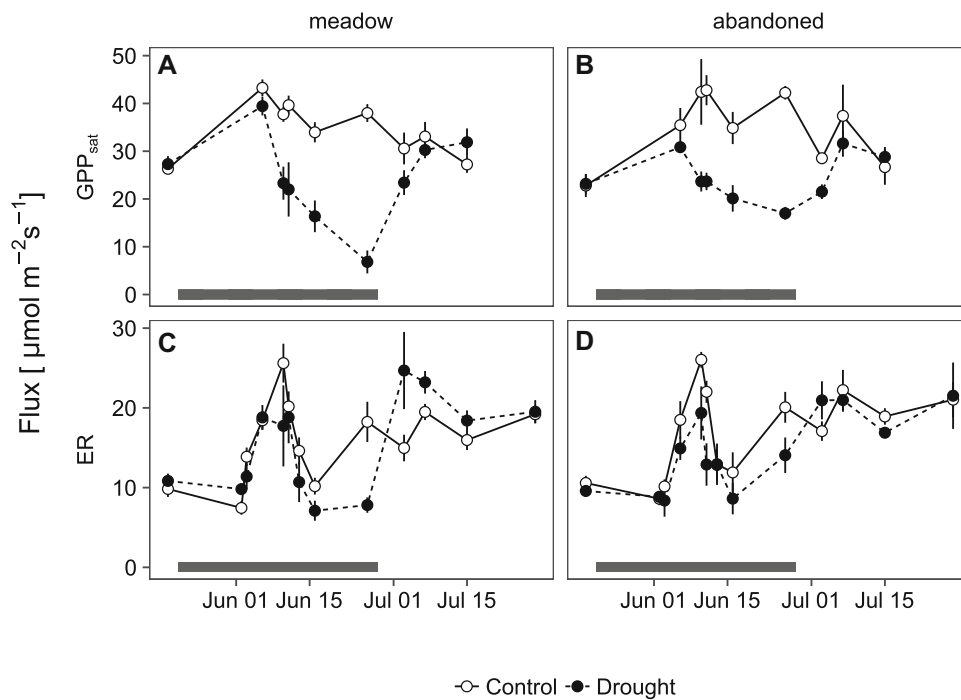
Figure 6. A, B Light-saturated rates of gross primary productivity ( GPP_{sat} ) and C, D ecosystem respiration (ER) in monoliths from the meadow and the abandoned grassland subjected to ambient conditions ( open symbols ) and drought ( closed symbols ). Error bars indicate standard errors of the mean ( n = 3–4). The horizontal black bars indicate the time of rain exclusion.
