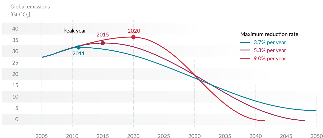
Figure 14: Possible emission paths for the 2°C goal (Source: Solving the climate dilemma, German Advisory Council on Global Change 2009)
