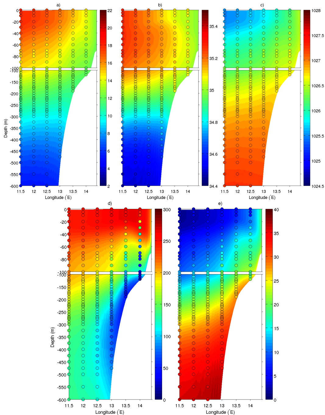
Fig. 5. Simulated 8 yr mean of (a) temperature ( ^{\circ}\text{C} ), (b) salinity, (c) density ( \text{kg m}^{-3} ), (d) oxygen ( \text{mmol O}_2 \text{m}^{-3} ) and, (e) nitrate ( \text{mmol N m}^{-3} ) concentrations at 23^{\circ}\text{S} between the surface and 600 m depth, with a zoom in the first 100 m depth. Colored circles for the annual mean CARS databases (2006, 2009) are overlaid on the simulated fields using the same color bar.
