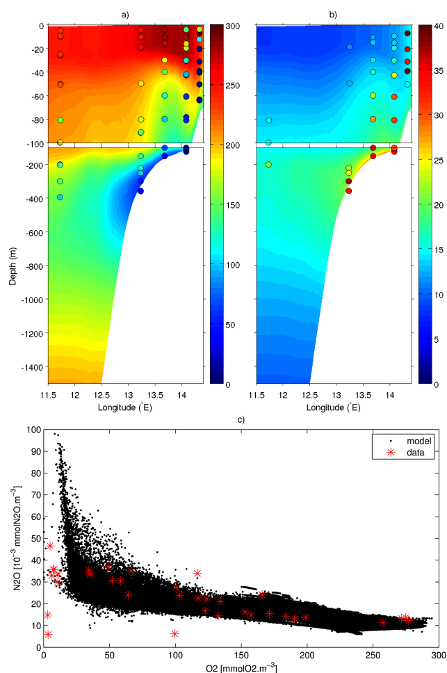
Fig. 9. (a) Oxygen ( \text{mmol O}_2 \text{m}^{-3} ), and (b) nitrous oxide ( 10^{-3} \text{mmol N}_2\text{O m}^{-3} ) concentrations estimated with the coupled model at 23^\circ \text{S} (averaged December over 8 yr) between the surface and 1500 m depth, with a zoom in the first 100 m depth. Colored circles for the FRS Africana (December 2009) data are overlaid on the modeled fields using the same color bar. (c) Nitrous oxide concentrations ( 10^{-3} \text{mmol N}_2\text{O m}^{-3} ) as a function of oxygen concentrations ( \text{mmol O}_2 \text{m}^{-3} ) at 23^\circ \text{S} . Black dots represent the simulated 3-day averaged fields for the whole analyzed period (Y12–Y19), and red stars in situ measurements from the FRS Africana cruise in December 2009.
