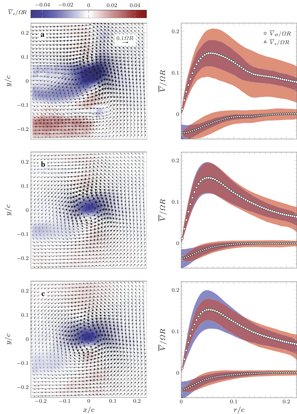
Fig. 7 Conditionally averaged vortex velocity fields (left) and the velocity profiles (right) at \psi = 1^\circ (a), 3^\circ (b), 5^\circ (c), 10^\circ (d), 20^\circ (e) and 30^\circ (f). The light red shading indicates deviations due to asymmetry ( \delta_1 V Eq. 4), the blue shading represents aperiodic deviations ( \delta_2 V Eq. 5) and the superposition of both is dark red
