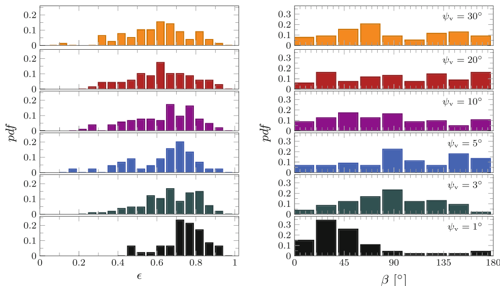
Fig. 5 Probability density function ( pdf ) of the vortex core eccentricity ( left ) and vortex core major axis orientation with respect to the horizontal ( right )
