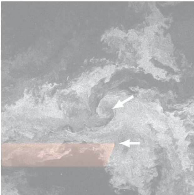
Fig. 3 An example of the tracer distribution within the region of interest at \psi_v = 3^\circ as seen by the lower camera; the blade is highlighted and the blade tip and vortex centre are indicated by the arrows
