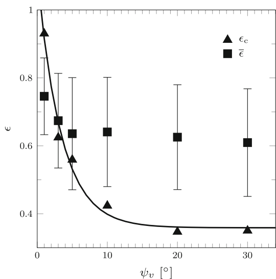
Fig. 6 The eccentricity \epsilon_c of the conditionally averaged vortices together with the conditional averaged eccentricity \bar{\epsilon} of the individual vortices; the solid line is a guide to the eye
