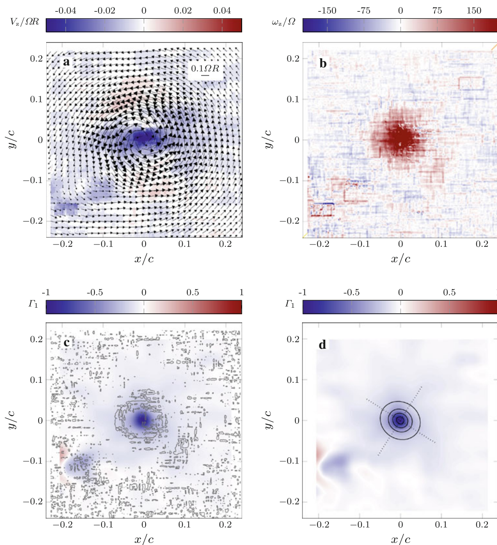
Fig. 2 A representative instantaneous velocity field (a) and the corresponding out-of-plane vorticity component (b) at \psi_v = 5^\circ . A combined representation of the scalar field \Gamma_1 (Eq. 1) and the contour lines of \lambda_2 = 0 for the same velocity field (c). The vortex core shape as derived by fitting Eq. 2 to \Gamma_1 where the dotted lines indicate the principle axes orientation (d)
