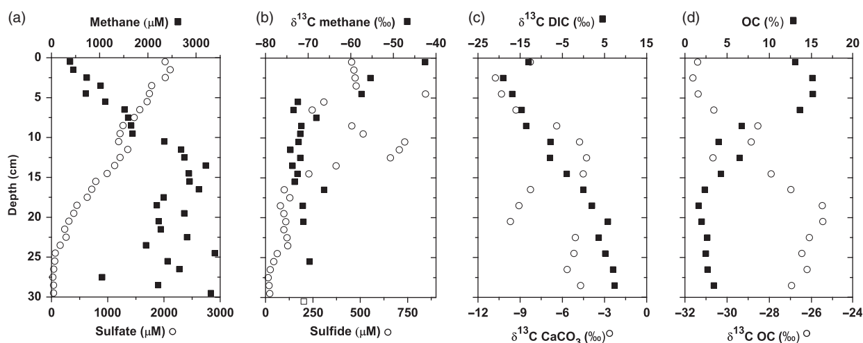
Fig. 1. Geochemical gradients in Lake Cadagno sediment core. (a) Methane and sulfate concentrations in \mu\text{M} . (b) Sulfide concentrations in \mu\text{M} and \delta^{13}\text{C} of methane (in \text{‰} vs. Vienna Pee Dee Belemnite, VPDB). (c) Carbon isotope values (in \text{‰} vs. VPDB) of dissolved inorganic carbon (DIC) and carbonate. (d) Organic carbon concentrations (% of dry weight) and carbon isotopic composition (in \text{‰} vs. VPDB).
