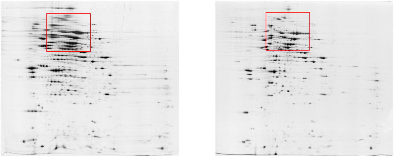
Fig. 16: 2DE protein profiles of D. toluolica Tol2 grown with phenylacetate. Immobilized pH gradient strips were rehydrated by rehydration buffer (left) and Destreak™ rehydration solution (right). Spot strings (examples indicated by red box) appear in both case. However, streaking effect was minimized when Destreak was used.
