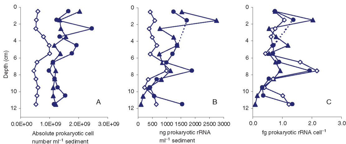
Fig. 3. Vertical profiles of total cell counts (panel A, mean of two parallel cores), prokaryotic rRNA recovery (B), and prokaryotic cellular rRNA content (C) in sandy Sylt sediments. The samples were collected in October 1999 (▲), March 2000 (◇) and July 2000 (●).
