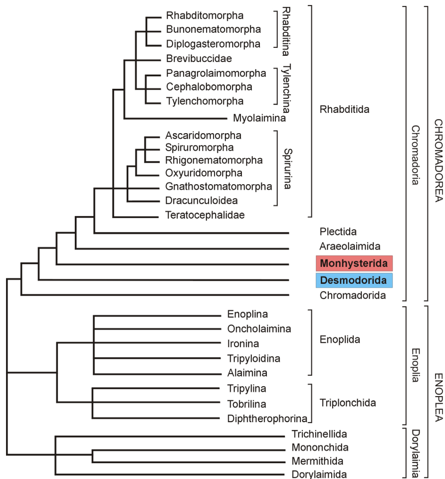
Fig. 2. Overview of the phylogenetic relationships among nematodes based on 18S rRNA gene sequence analyses. Nematode orders with members that are involved in symbiotic associations are highlighted. Modified from De Ley & Blaxter, 2002.
