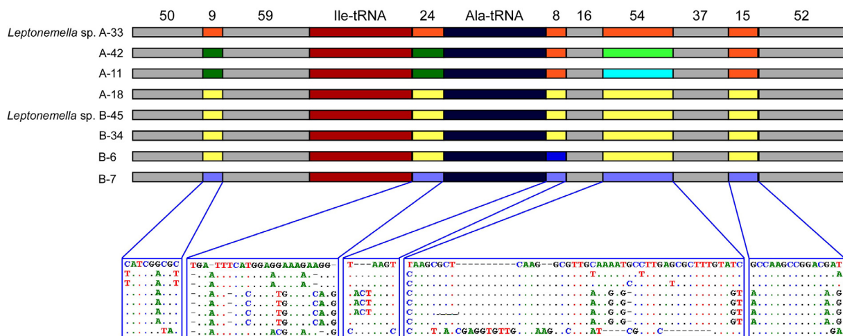
Fig. 3. Mosaic-like structure of ISR sequences of the symbionts of Leptonemella species A and B. The grey colour represents sequence blocks that are identical in ISR of all symbionts investigated. Other colours indicate sequence blocks that varied between different individuals. The sequence information of the variable regions is shown as alignment. Nucleotide positions that are conserved are indicated by dots. Gaps that have been included to obtain optimal sequence alignment are indicated by dashes. Identical fragments between sequences are denoted by the same colour. Two tRNA genes (for Ile and Ala) were found in all symbiont's ISR sequences. The numbers above columns represent sequence length in bp.
