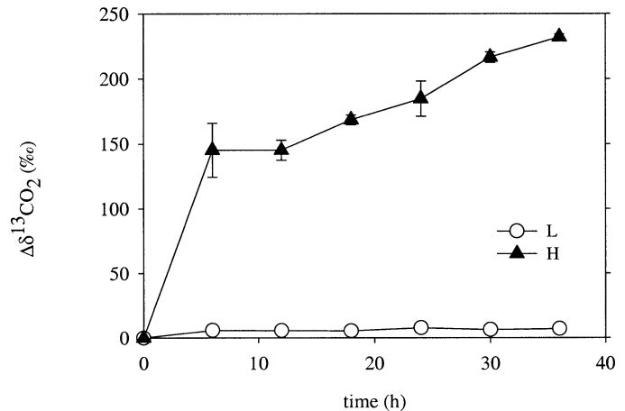
Fig. 2. ^{13}C enrichment in \Sigma\text{CO}_2 [%] in the overlying water versus time for the L and H experiments. Error bars represent the range of two replicates.
