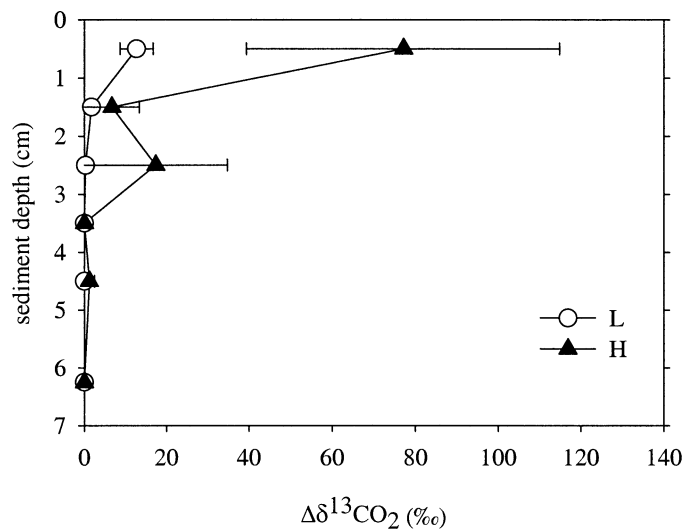
Fig. 3. ^{13}C enrichment in \Sigma\text{CO}_2 [%] in the pore-water versus sediment depth for the L and H experiments after 36 h. Horizontal bars indicate the range of two replicates.
