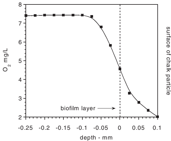
Figure 2 Microsensor oxygen profile of biofilm covered chalk particle
