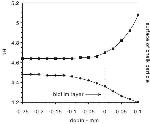
Figure 1 Microsensor pH profiles of virgin chalk (■) and biofilm covered chalk particles (●)
