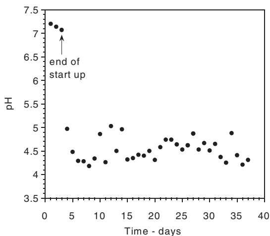
Figure 3 Sintered glass reactor pH
