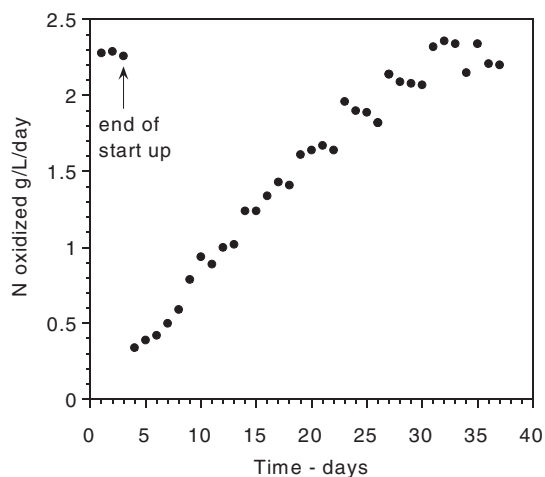
Figure 4 Sintered glass reactor nitrification performance at low pH
