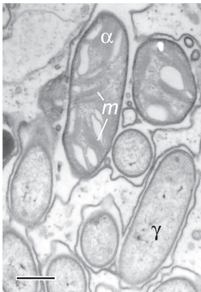
Figure 3. Cross section of the dorsal area of a gill filament where both morphotypes of symbiotic bacteria co-occur (TEM). \gamma = abundant chemoautotrophic morphotype, \alpha = second morphotype with stacks of internal membranes ( m ) resembling those of type I methanotrophs. Scale 0.5 \mu\text{m} .
