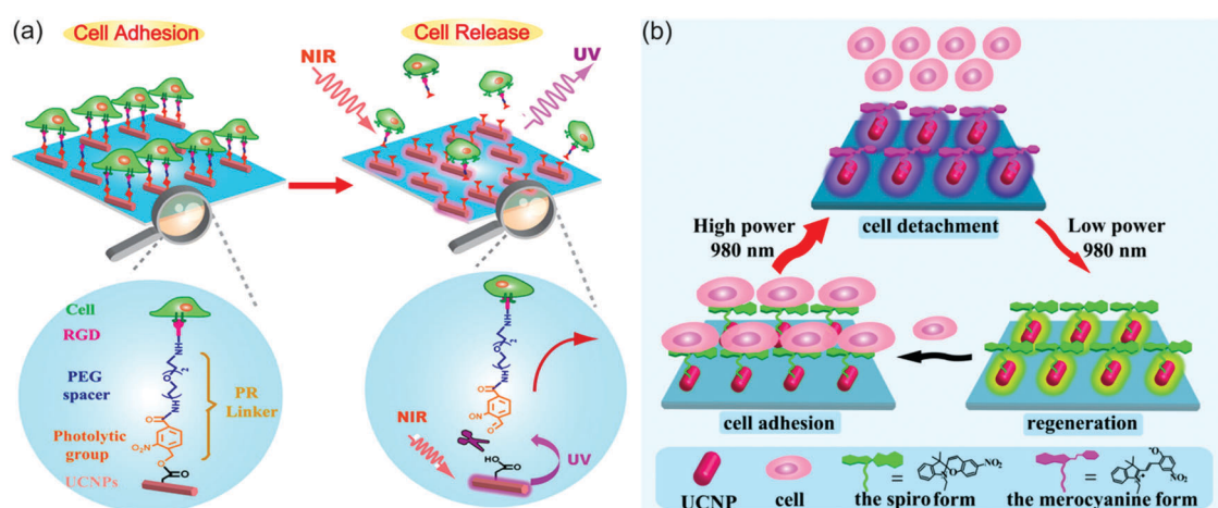
Fig. 12 (a) Irreversible control of cell adhesion using NIR light based on UCNPs. Upon 980 nm light excitation, the UCNPs emit UV photons, which cleave the photolytic linker. As a result, the cells dissociate from the substrate. (b) Reversible control of cell adhesion/detachment using NIR light with different intensities based on UCNPs. At a high intensity ( 8 \text{ W cm}^{-2} ), the UCNPs emit UV photons and activate the isomerization from the spiropyran form to the merocyanine form, resulting in the cell detachment. Conversely, when exposed to a low intensity ( 0.5 \text{ W cm}^{-2} ), the same UCNPs can emit visible light to drive the merocyanine form back to the spiropyran form, leading to cell adhesion again. Panel (a) reproduced with permission. 90 Copyright 2014, American Chemical Society. Panel (b) reproduced with permission. 65 Copyright 2015, American Chemical Society.
