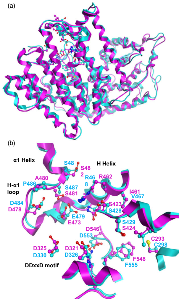
Figure 5 Structural analysis of GmAFS. (a) Supposition of the homology models for GmAFS (magenta) and MdaAFS (cyan). The two models can be superposed well with a RMSD deviation of 1.5 Å. The active site residues are shown in ball and stick. (b) The active site structures and residues from the GmAFS and MdaAFS models. H- \alpha 1 loop, DDxxD motif and H helix are also shown.
