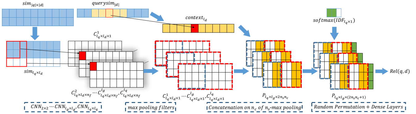
Figure 1: The pipeline of RE-PACRR. The inputs include two matrices, namely, sim_{|q| \times |d|} and querysim_{|d|} , recording the similarity of different terms in a document relative to each query term and the whole query respectively. All these similarity matrices are truncated/zero-padded to the dimensions governed by l_q and l_d . Several 2D convolutional kernels are first applied to the similarity matrices, one for each l_g \in [2, l_g] , and an extra one for query proximity with kernel size l_q \times l_q . Next, max pooling is applied to pool out the filters, ending up with l_g + 1 matrices, namely, C^1 \dots C^{l_g}, C^{l_q} . Following this, n_s -max pooling captures the strongest n_s signals on each C , at all n_c positions from cpos . In the meantime, the context similarity corresponding to each term in top\text{-}n_s from context_{l_d} is also appended, leading to P_{l_q \times l_g \times (2n_s n_c)} . Finally, the query terms’ normalized IDFs are appended, and a feedforward network is applied, after permuting the rows in P_{l_q \times l_g \times (2n_s n_c + 1)} , getting a query-document relevance score rel(q, d) . In this plot, the situation when l_d = 8, l_q = 3, l_g = 3, n_c = 2, n_s = 2 and cpos = [50\%, 100\%] is displayed.
