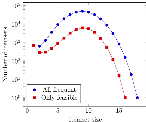
Figure 2: The number of frequent itemsets and feasible frequent itemsets when solving the \text{MAXFS}(\mathbf{G}) problem using MAXFIS algorithms. The y -axis is in logarithmic scale.
