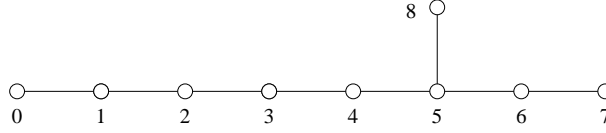
Figure 1: The Dynkin diagram of \epsilon_9 .
