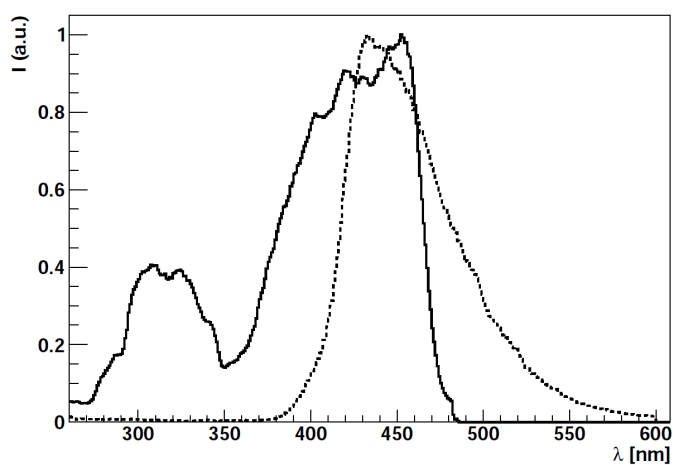
Figure 6.5: Absorption spectrum of BCF-91A fiber (solid line) and emission spectrum of TPB (dashed line). Figure taken from [94].
