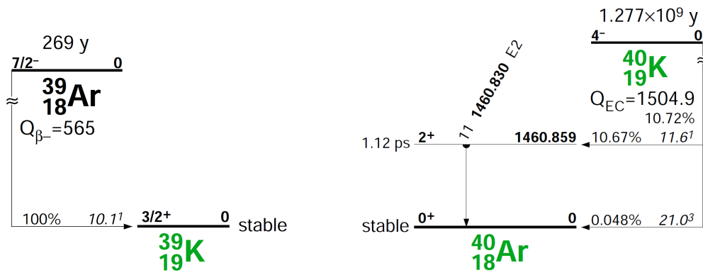
Figure C.2: Decay scheme of ^{39}\text{Ar} [69].
