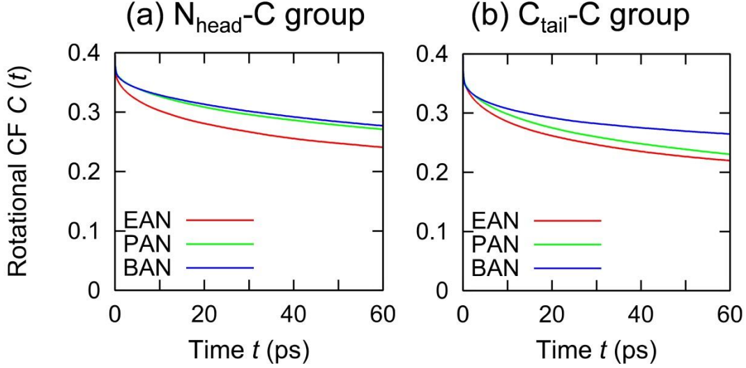
Figure 5.2. (a) N_{\text{head-C}} rotational correlation functions and (b) C_{\text{tail-C}} rotational correlation functions for ethylammonium nitrate (EAN; red), propylammonium nitrate (PAN; green), and butylammonium nitrate (BAN; blue) at 298.15 K.
