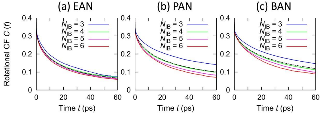
Figure 5.6. N_{\text{head}}\text{-H} rotational correlation functions for different number of the inter-ionic N_{\text{head}}\cdots N_{\text{anion}} bonds ( N_{IB} = 3 (blue), 4 (green), 5 (pink), and 6 (red)) for (a) ethylammonium nitrate (EAN), (b) propylammonium nitrate (PAN), and (c) butylammonium nitrate (BAN) at 298.15 K. The dashed black lines denote the original rotational correlation functions shown in Figure 1(a).
