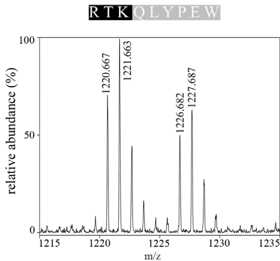
Figure 3. Generation of PSP by proteasomal trans splicing. (A) To demonstrate the generation of a PSP trans by the binding of two fragments originated from two distinct molecules of substrate, 5 nmol gp100 40-52 and its heavy analogue with amino acids 13 C 6 -Lys and 15 N-Leu (RTK 6 AWNRQL 1 YPEW) were digested together for 36 hours by 1.5 μg LcL 20S proteasomes in 100 μl buffer. Theoretically four different PSP could be generated from the cis or trans ligation of the proteasomal fragments [RTK] and [QLYPEW] with sequences [RTK][QLYPEW]: gp100 40-42/47-52 -α, [M+H] + = 1220.7; gp100 40-42/47-52 -β, [M+H] + = 1221.7; gp100 40-42/47-52 -γ, [M+H] + = 1226.7; gp100 40-42/47-52 -δ, [M+H] + = 1227.7. (B) LC-MALDI-TOF/TOF-MS spectra at RT = 41.3 min show peaks which can be assigned to all four possible PSP of gp100 40-42/47-52 (for MS/MS spectra see Figure S1). doi:10.1371/journal.pcbi.1000830.g003
