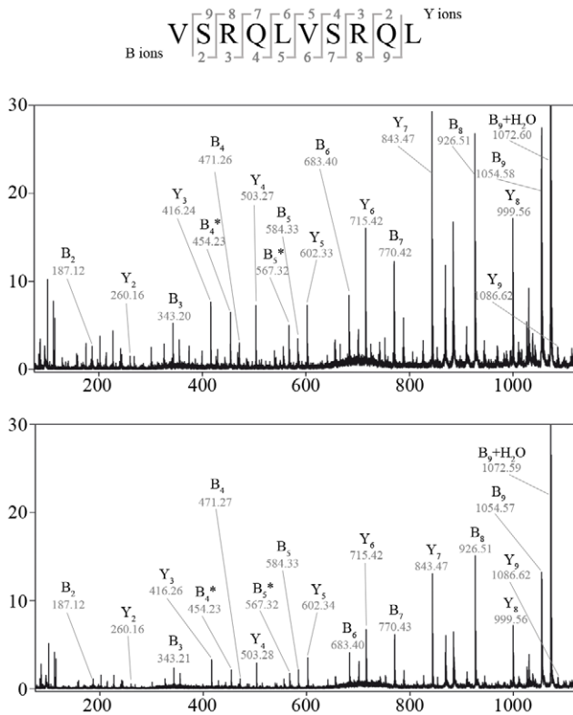
Figure 5. MS/MS identification of the PSP trans gp100 35-39/35-39 [VSRQL][VSRQL] within the gp100 35-57 digestion products. MALDI-TOF/TOF-MS/MS spectrum of precursor ion [M+H] + = 1185.7 observed in the up-scaled digestion (see “Methods” section) of the 23mer gp100 35-57 by 205 LcL proteasomes (upper panel) is shown in comparison with the synthetic peptide [VSRQL][VSRQL] (lower panel). In the spectra B-, Y-ions, the loss of ammonia symbolized by *, the relative abundance (%) in y-axis and m/z in the x-axis, are reported. doi:10.1371/journal.pcbi.1000830.g005
