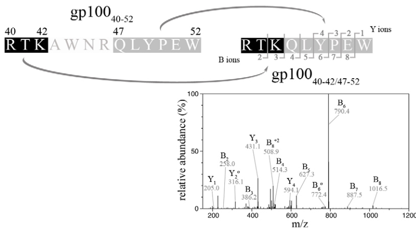
Figure 2. By applying SpliceMet we identified the known PSP produced by digestion of the synthetic 13mer gp100 40-52 by 20S proteasomes. Sequence of the substrate gp100 40-52 and of the PSP gp100 40-42/47-52 and its ESI-MS/MS spectrum (double protonated with m/z 610.8) are shown. In the spectra B- and Y-ions are reported. Ions' loss of water is symbolized by °. In the experiments (100 \mu l of reaction) 4 nmol of gp100 40-52 were cleaved for 36 hours by 1 \mu g 20S proteasome purified from LcL.
