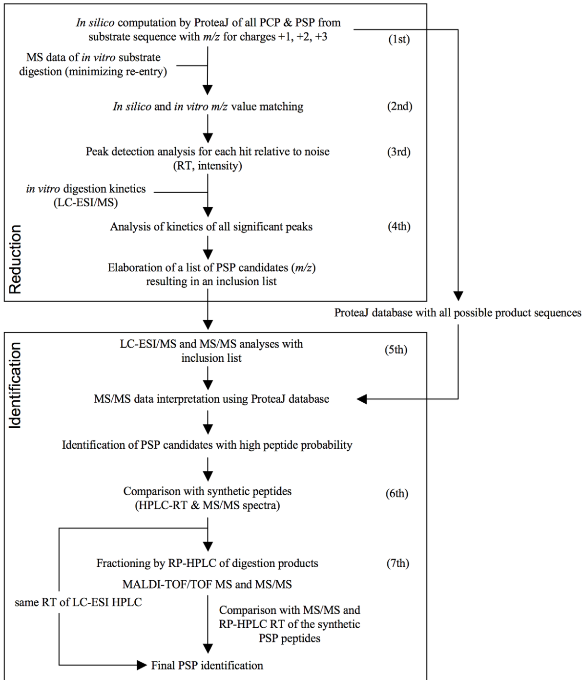
Figure 1. SpliceMet. Applying the computer program ProteaJ on a peptide sequence of choice, m/z values of all theoretically possible proteasomal cleavage (PCP) and splicing (PSP) products are calculated (1 st step). This is followed by an in vitro digest of the synthetic substrate and the comparison of the obtained MS signals with the theoretical m/z values (2nd). Matching of the signals and verification of peptide generation kinetics results in an inclusion list for LC-ESI-MS/MS analysis required for identification of the PSP (3rd, 4th). For final confirmation, the MS/MS spectra (5th) and the HPLC-RT of proposed PSP (6th) are compared with those of the analogous synthetic peptides. For the identification of those PSP candidates that do not fully satisfy these requisites, the generation of PSP is up-scaled followed by HPLC fractionation with an extended gradient and the fractions are analyzed by nano-LC-MALDI-TOF/TOF-MS (7th). doi:10.1371/journal.pcbi.1000830.g001
