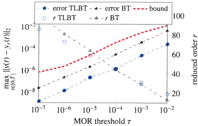
Figure 3. Automatically adjusted orders r , maximum errors, bound (10) against tolerances \tau for the larger rail model ( n = 79841 , \bar{T} = 150 , u(t) = u_*(t) ).
