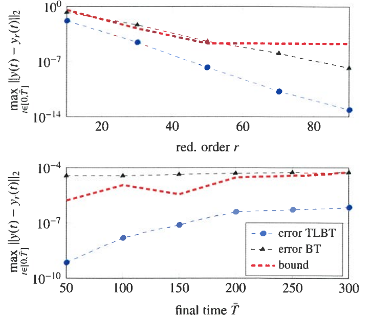
Figure 2. Influence of r (top) and \bar{T} (bottom) for small rail model.
