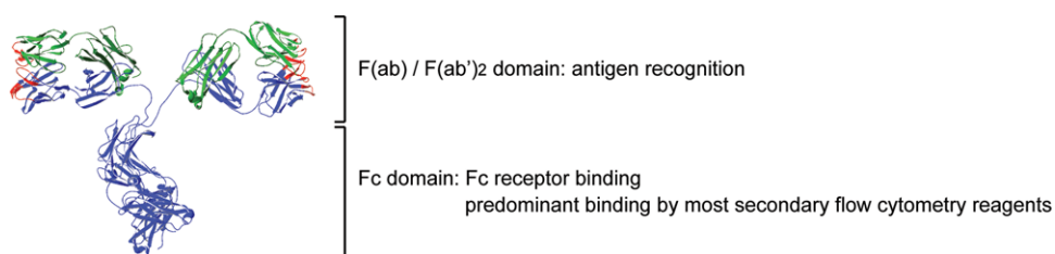
Figure 33. Structural characteristics of immunoglobulins. Ribbon diagram of a mouse monoclonal IgG antibody consisting of two identical heavy and light chain proteins, respectively. Antibody heavy chain residues are indicated in blue and light chain residues in green. Amino acid residues encoding the CDR1, 2 and 3 regions are shown in red. (Image was generated using the Swiss PDB viewer and PDB accession number 1IGT).
