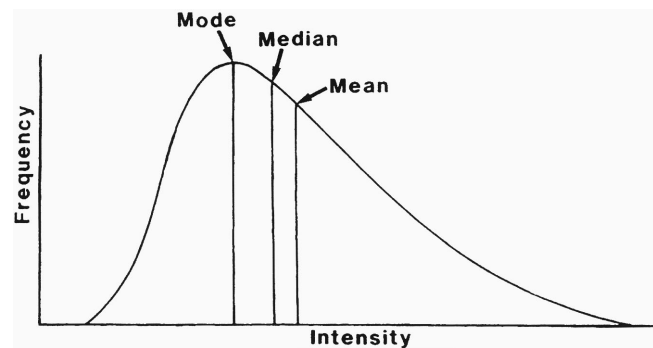
Figure 40. Measurements of central tendencies for cytometric intensity histograms. The curve is an ideal distribution, showing key measurements. Cytometric intensity histograms span a finite intensity range with a noisy curve and frequently with off-scale events at the lower and/or upper end(s) of the scale. Generally the median is the most robust measure, because the mean is heavily influenced by off-scale events and the mode by noise.
