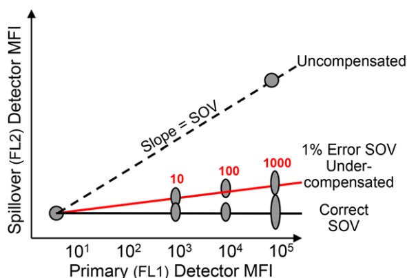
Figure 16. Brightness of positive population.
