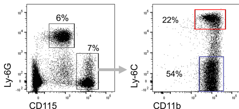
Figure 107. Flow cytometric analysis of murine myeloid blood cells. Neutrophils are defined by high sideward scatter (not shown) and expression of Ly6G. Monocytes are defined as CD115 hi cells and can be further subdivided into classical (Ly6C hi ; red) and patrolling monocytes (Ly6C lo ; blue) (for further details see [850]).
