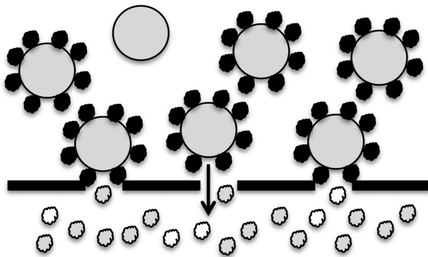
Figure 23. Unlabelled cells will pass the mesh without any (enrichment) effect (A). If you add beads which are coated with specific antibodies against your target cells (black) to the cell suspension, the target cells will form aggregates with the beads. These aggregates are held back on the top of the mesh while the rest of the cell suspension is passes through (B). With this method one can either deplete or enrich for a specific cell population. Combining different mesh and bead sizes allows for a serial enrichment of target cells.
