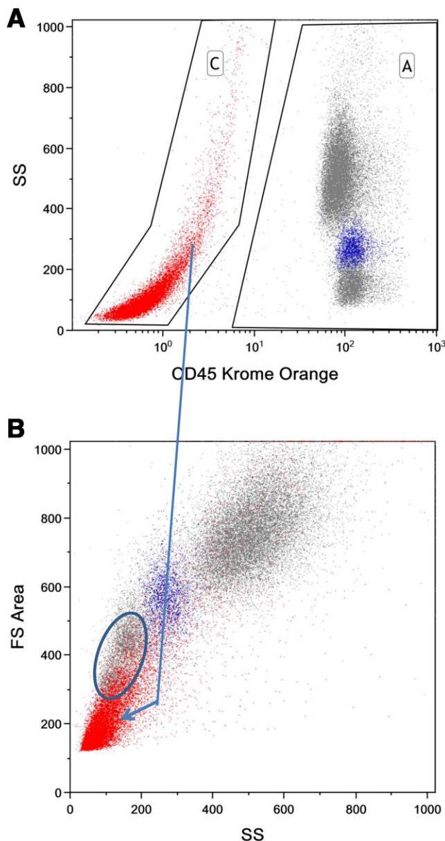
Figure 26. Human whole blood fixed with formaldehyde and permeabilized with TX-100. White blood cell populations are identified using CD14-PE-Cy7 and CD45-Krome Orange. Debris (red) is identified using CD45 vs SS (top panel - region C). Identification of peripheral blood monocytes (shown in blue in both panels) was accomplished using CD-14-PE-Cy7 (not shown).
