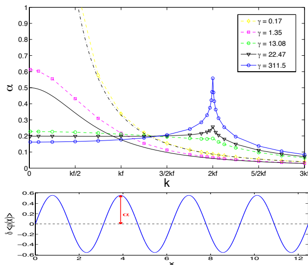
Figure 1: Top: The response amplitude \alpha = \max_x \delta \langle \rho(x) \rangle for different values of \gamma = g/\rho as a function of the momentum k . The dashed and solid line without markers are the classical Bogoliubov results for \gamma = 0.17 and \gamma = 1.35 respectively. Bottom: Density fluctuation \delta \langle \rho(x) \rangle = \langle \rho(x) \rangle - \rho at \gamma = 311.5 and k = 2k_F . All calculations in both panels were done with cMPS bond dimension D = 64 .
