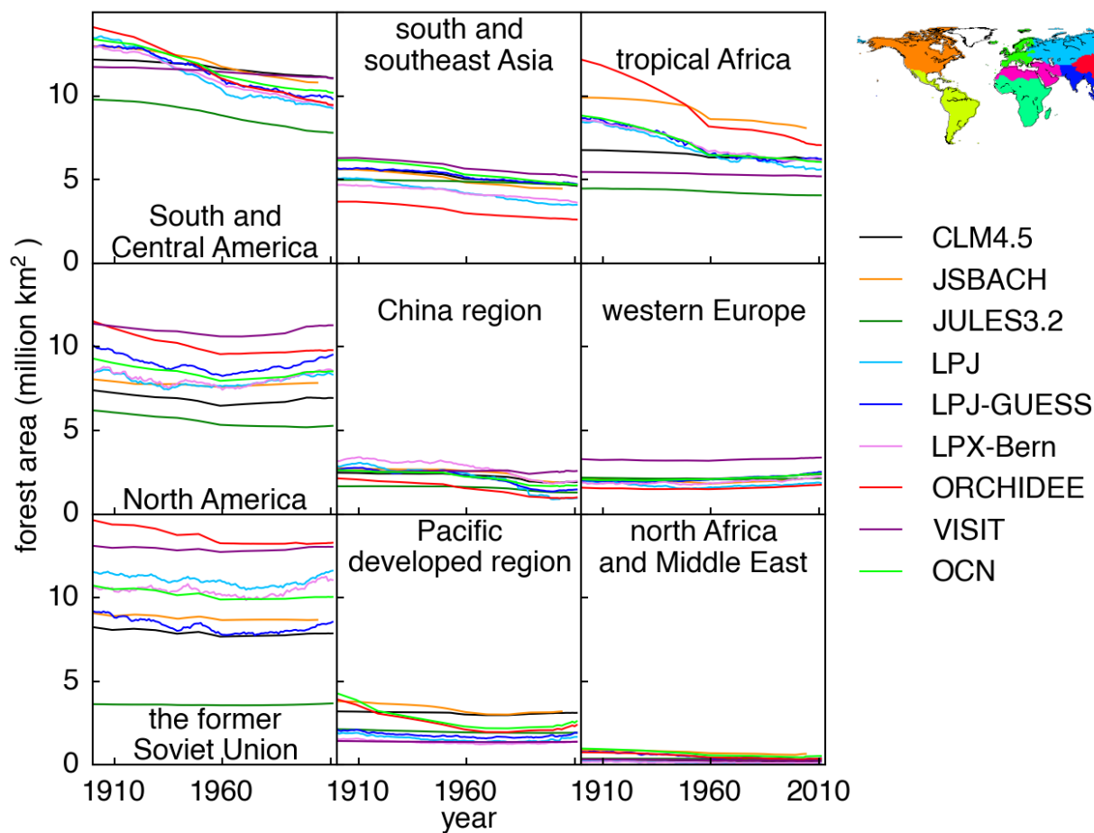
Figure 2. Temporal change of forest area from TRENDY v2 models in each of the nine regions. Differences between models arise from their specific vegetation maps and rules through which natural PFTs are chosen to give land to agriculture.
