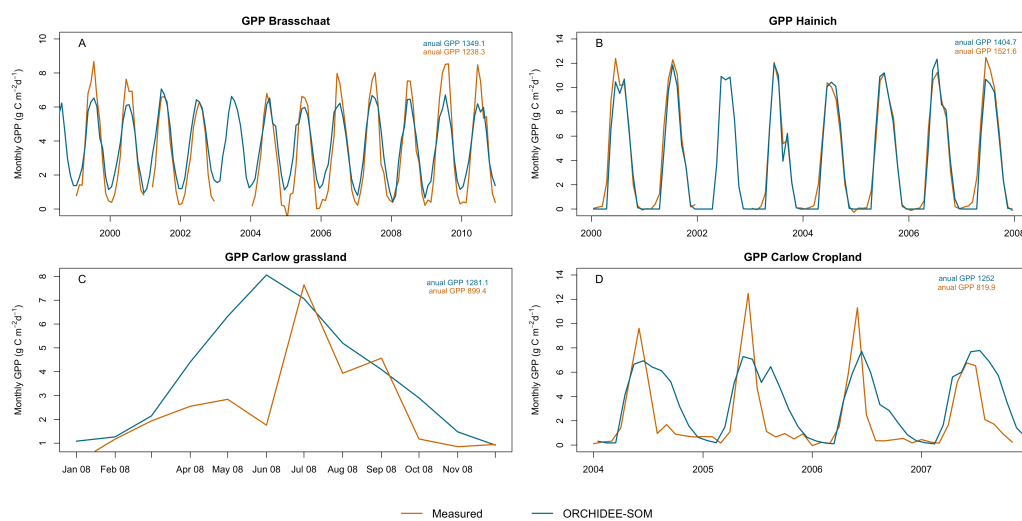
Figure 2. Measured and modelled daily GPP (monthly means) at the four sites, (A) Brasschaat forest, (B) Hainich forest, (C) Carlow grassland and (D) Carlow cropland, after GPP optimization. Measured GPP are acquired from each FLUXNET site and modelled GPP was acquired using ORCHIDEE-SOM.
