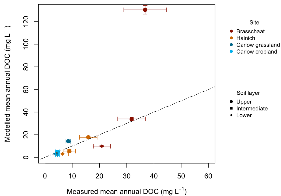
Figure 8. Measured versus modelled mean annual DOC concentrations ( \text{mg C L}^{-1} ). Error bars represent the standard deviations for the mean annual DOC concentrations. The dashed line represents the 1:1 line.
