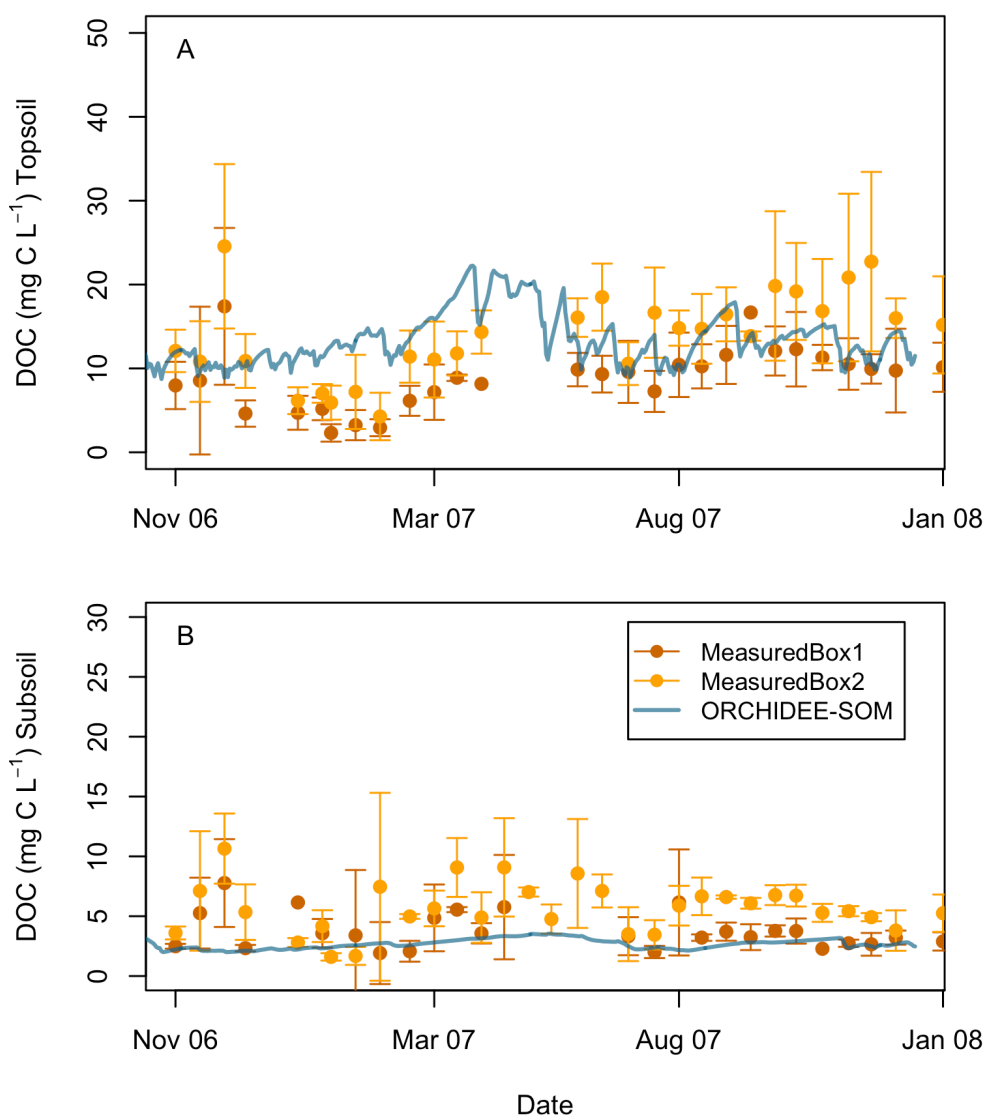
Figure 6. ORCHIDEE-SOM simulated (daily values) and measured DOC dynamics at Carlow grassland at two soil layers, (a) topsoil, 10-30 cm; and (b) subsoil, 60-75 cm. Site measurements are in brown for Box 1 and in orange for Box 2, and simulation results using ORCHIDEE-SOM (daily values) in blue. Error bars represent the standard deviation of site measurements (n=5).
