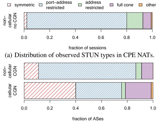
(a) Distribution of observed STUN types in CPE NATs. (b) Most permissive STUN type per AS (only CGN sessions).
