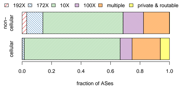
(a) Internal address space usage per CGN deployment.
