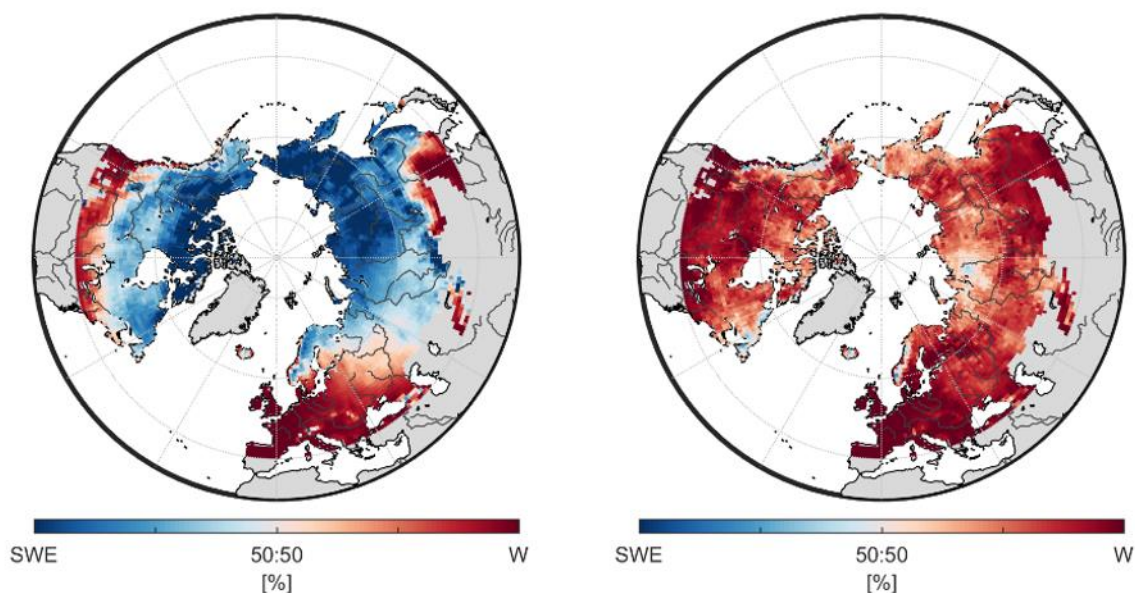
Figure 7. Relative contribution based on CR (Eq.(3)) of modelled snow (SWE) and liquid water (W) storage anomalies to a) mean seasonal variations from 2000–2014 of modelled TWS anomalies, and b) inter-annual variations of modelled TWS anomalies for each grid cell of the study domain, respectively.
