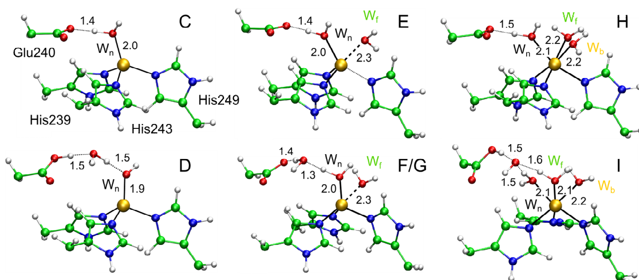
Figure 20: Coordination of zinc at the catalytic site of an uninhibited MT1-MMP: models C-I.
